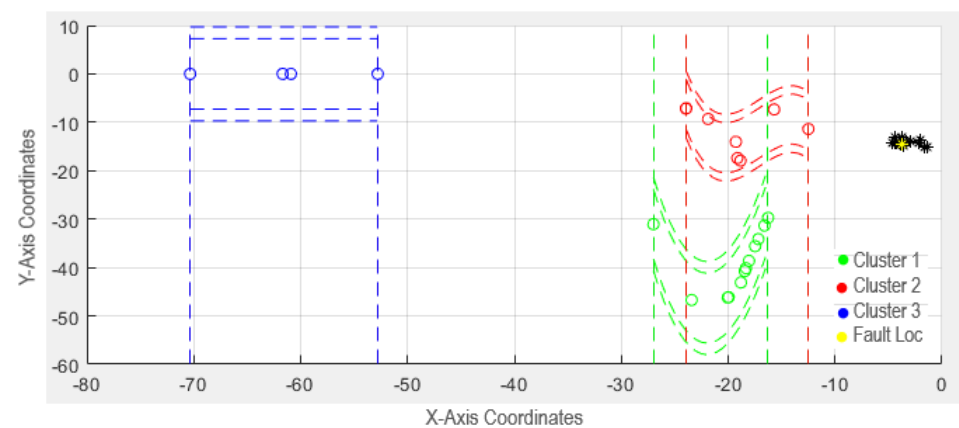
Figure 16. 100 \Omega fault identified.
