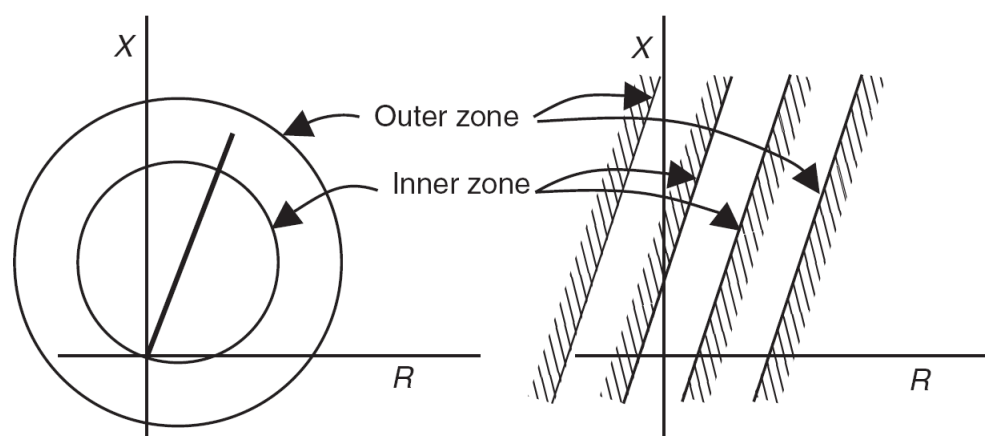
Figure 2. Out of Step Relay characteristics [26].
