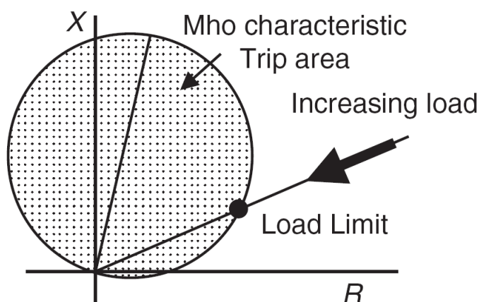
Figure 1. Mho Relay Characteristic [26].
