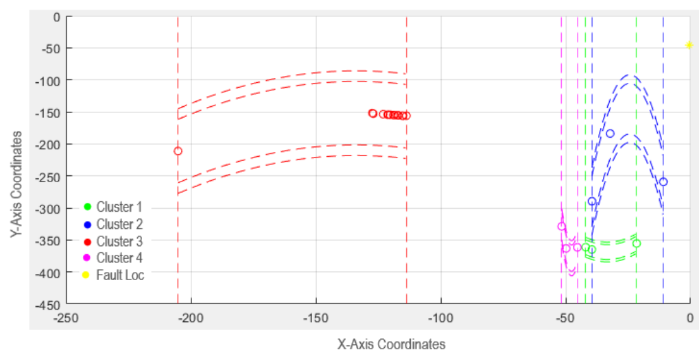
Figure 20. 10\ \Omega fault identified.
