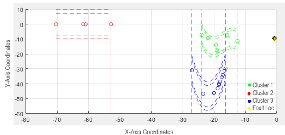
Figure 15. 10 \Omega fault identified.
