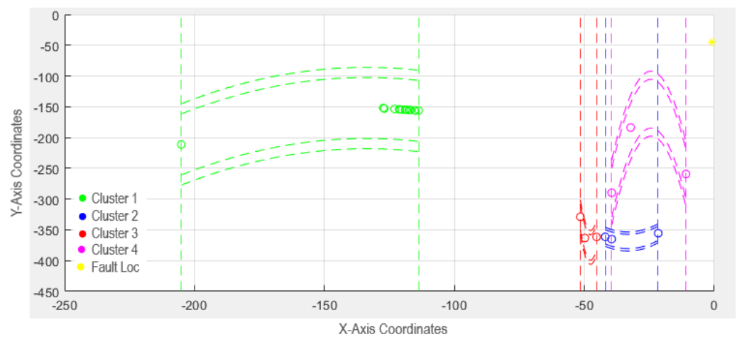
Figure 21. 100 \Omega fault identified.
