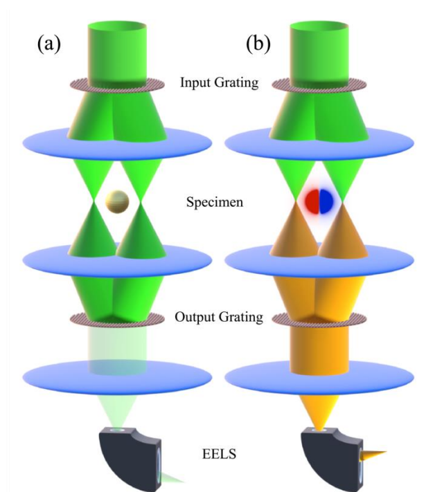
Figure 1. Illustration of 2GMZI elastic ZLP component; right, dipole plasmon scattered component resolved with an EELS spectrometer. Illustration of 2GMZI for the (a) elastic ZLP component, and the (b) dipole plasmon scattered component resolved with an EELS spectrometer.
