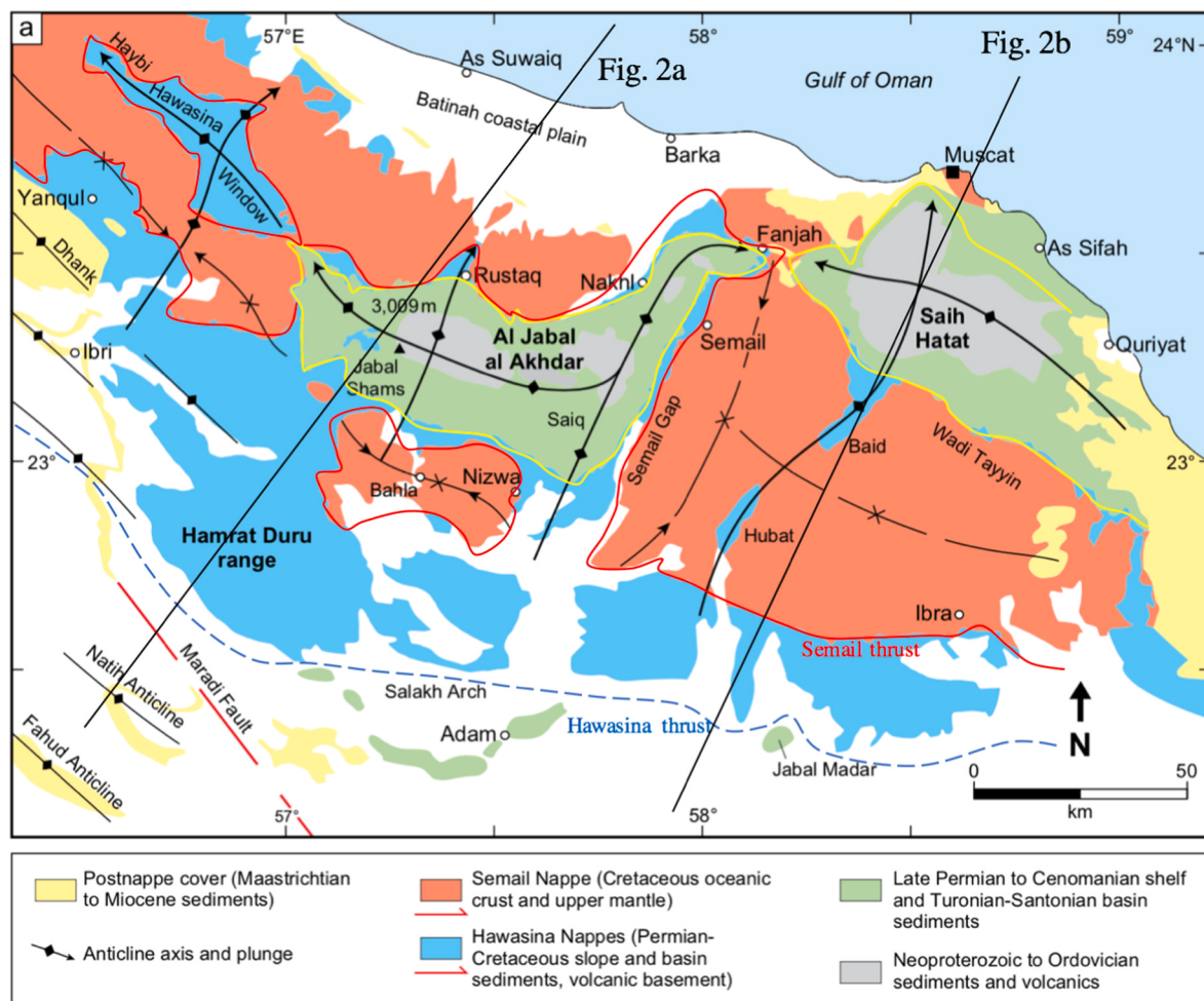
Fig. 1. Geological map of the Jebel Akhdar and Saih Hatat culminations in the central part of the Oman Mountains, showing key geological features. Red line is the Semail Thrust ( sensu stricto ). Dashed blue line is the SW limit of the Hawasina thrust sheet. Yellow lines are the low-angle normal faults surrounding the shelf carbonate inliers (or windows) of Jebel Akhdar and Saih Hatat. (For interpretation of the references to colour in this figure legend, the reader is referred to the Web version of this article.)
