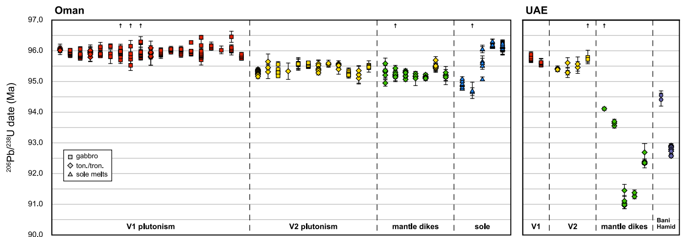
Fig. 5. Summary of high-precision U–Pb zircon dates from our previous work (Rioux et al., 2012, 2013, 2016, 2021; Searle et al., 2015). The data provide a large, internally consistent dataset that precisely dates the different magmatic and metamorphic events within the ophiolite. Each datum is the date from a single zircon grain or grain fragment ( \pm 2s ), and vertical clusters of dates are from a single sample. Samples within each division are arranged from south to north. Dates from the Oman sole exposures are from four leucocratic pods (tight clusters) and a single garnet amphibolite. Small arrows at the top of the figure indicate that the sample contains one or more xenocrystic zircon grain(s) that plot off-scale.
