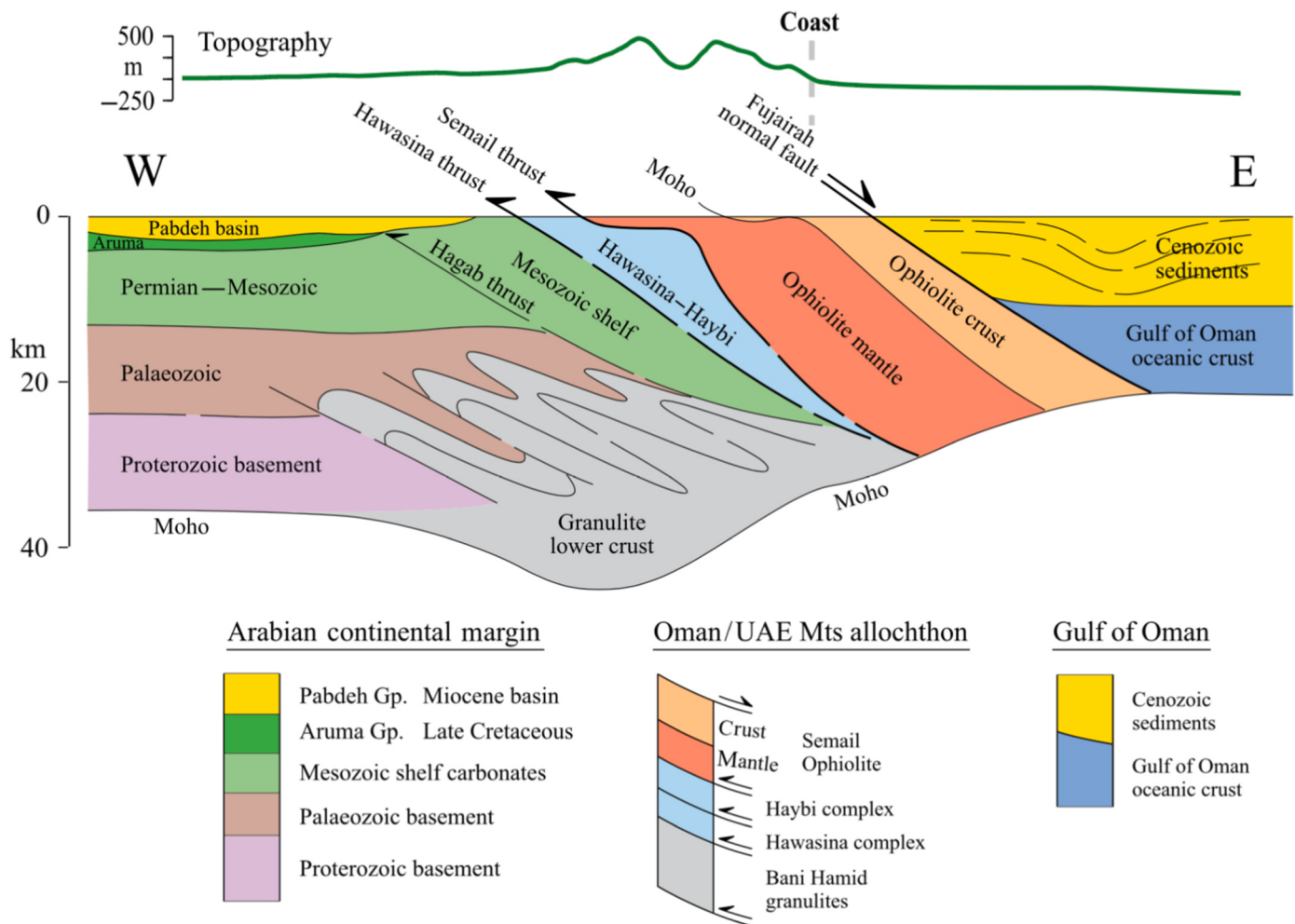
Fig. 9. Simplified section across the UAE part of the north Oman Mountains, after Ali et al. (2020), showing structural interpretation of surface geology combined with deep seismic profiles. The Semail Thrust structurally overlies the allochthonous Haybi and Hawasina thrust sheets. The eastern margin of the ophiolite is a ENE-dipping normal fault detaching the ophiolite from the in situ Gulf of Oman crust. The lower crust is interpreted as folded and thickened granulite facies rocks as exposed in the Bani Hamid thrust sheet.
