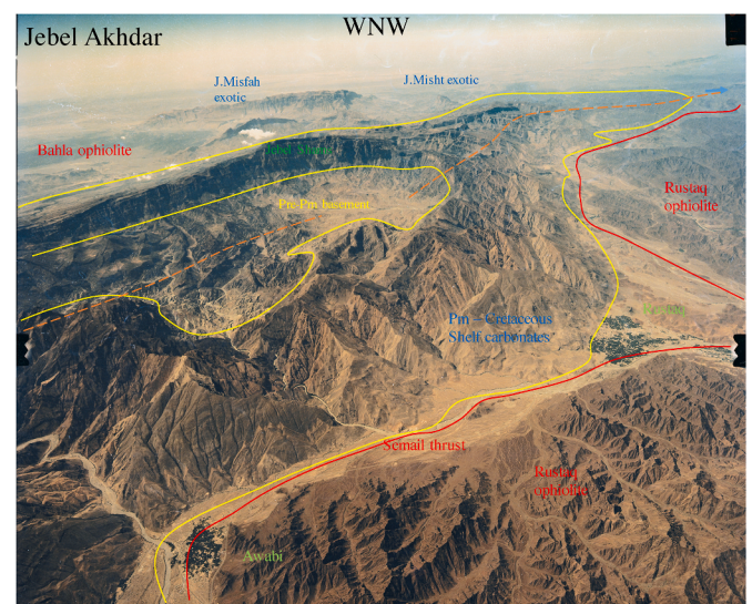
Fig. 11. Aerial photo of the giant Jebel Akhdar dome, view towards the WNW showing the Semail Thrust (red) folded over the anticline, and reactivated as a low-angle normal fault (yellow) during compressional uplift of Jebel Akhdar. Photo courtesy of Petroleum Development (Oman) Ltd. (For interpretation of the references to colour in this figure legend, the reader is referred to the Web version of this article.)
