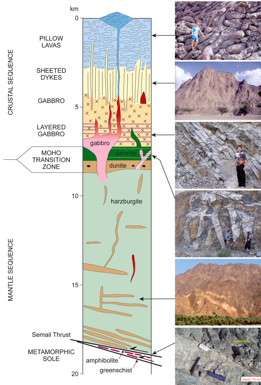
Fig. 4. Generalised section through the entire upper mantle and crust section of the Semail ophiolite, after Searle et al. (2014). The original Semail Thrust along the base of the mantle sequence is the initial obduction-related thrust fault.
