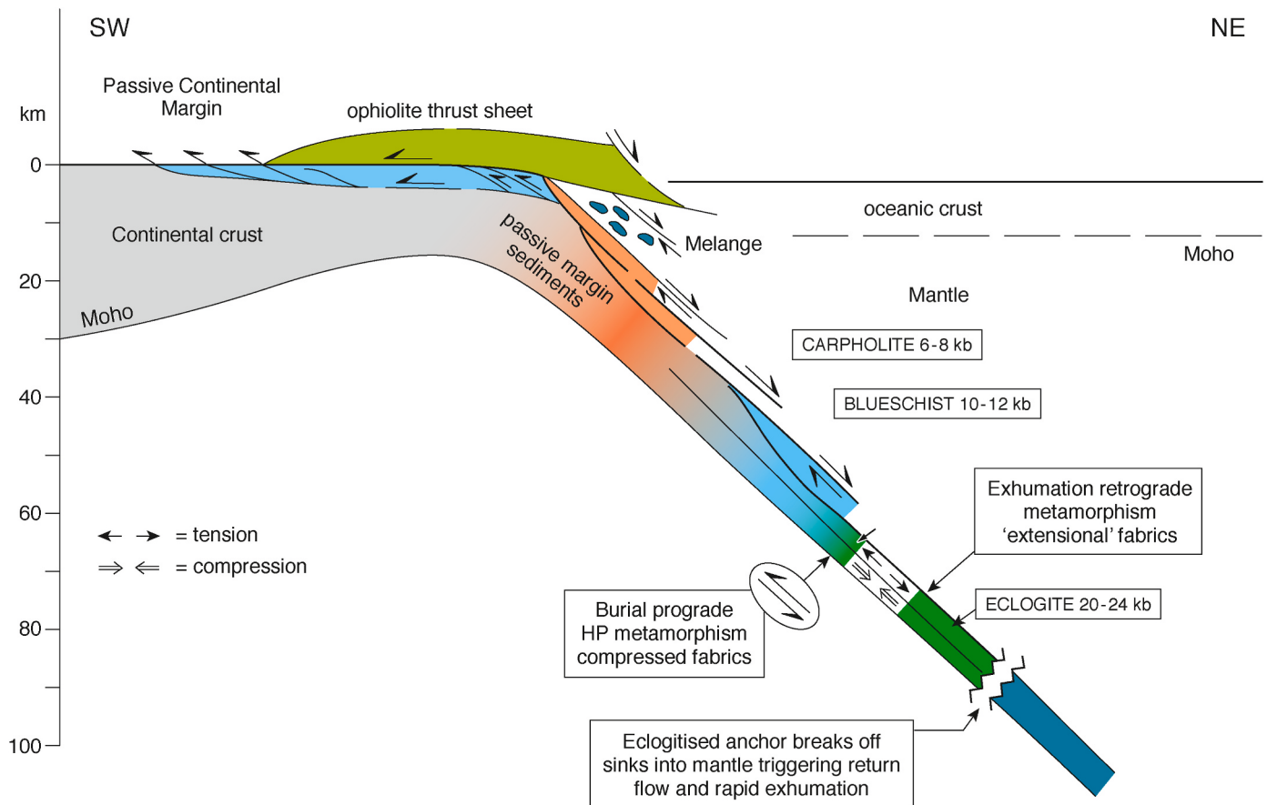
Fig. 10. Simplified section across the Muscat – As Sifah part of the north central Oman Mountains, showing a reconstruction of the HP rocks of As Sifah eclogites, Hulw blueschists, and Ruwi mélange units, using pressures to constrain depth. The Muscat ophiolite was continuous with the main Semail ophiolite at this stage at ca 79 Ma, the timing of peak eclogite facies metamorphism. Note the ‘extensional’ fabrics related to exhumation of footwall rocks along each thrust sheet. The Semail Thrust forms a passive roof fault above the Ruwi mélange.
