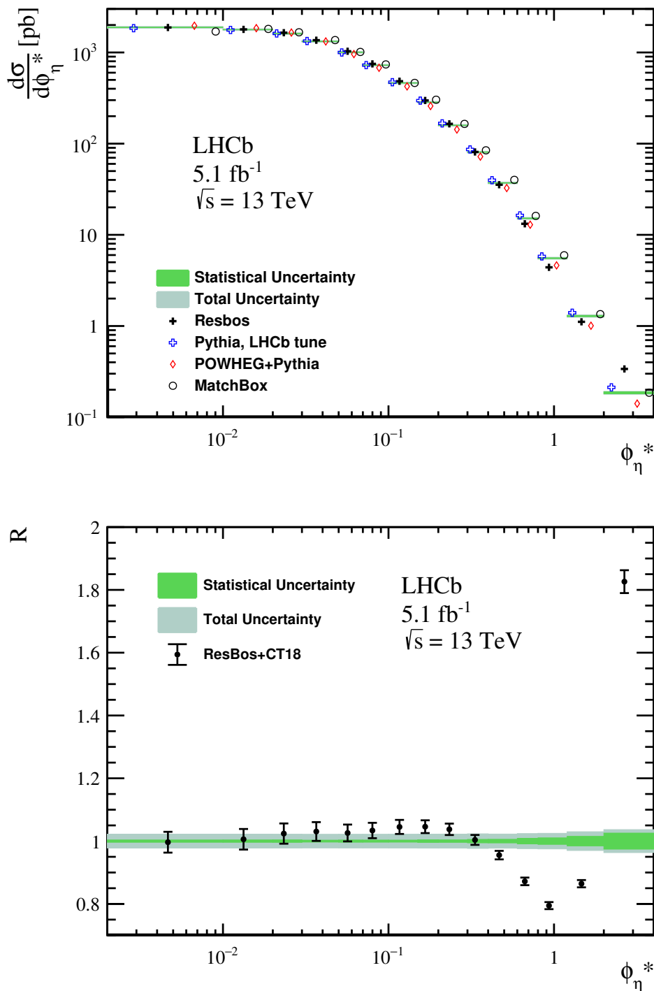
Figure 5. (Top) Measured single differential cross-section in regions of \phi_\eta^* , compared with different theoretical predictions. (Bottom) Ratio of RESBOS predictions to measurement, with the horizontal bars showing the uncertainty from the PDFs.
