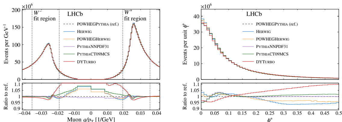
Figure 10. Projections of the (left) q/p_T and (right) \phi^* distributions for the challenge datasets. The four dashed vertical lines indicate the two fit regions in the q/p_T distribution.
