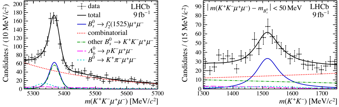
FIG. 3. Reconstructed invariant mass of (left) the K^+K^-\mu^+\mu^- system and (right) the K^+K^- system for B_s^0 \rightarrow f_2'(1525)\mu^+\mu^- candidates, overlaid with the fit projections. The m(K^+K^-) distribution is shown in the B_s^0 signal region \pm 50 MeV/ c^2 around the known B_s^0 mass.
