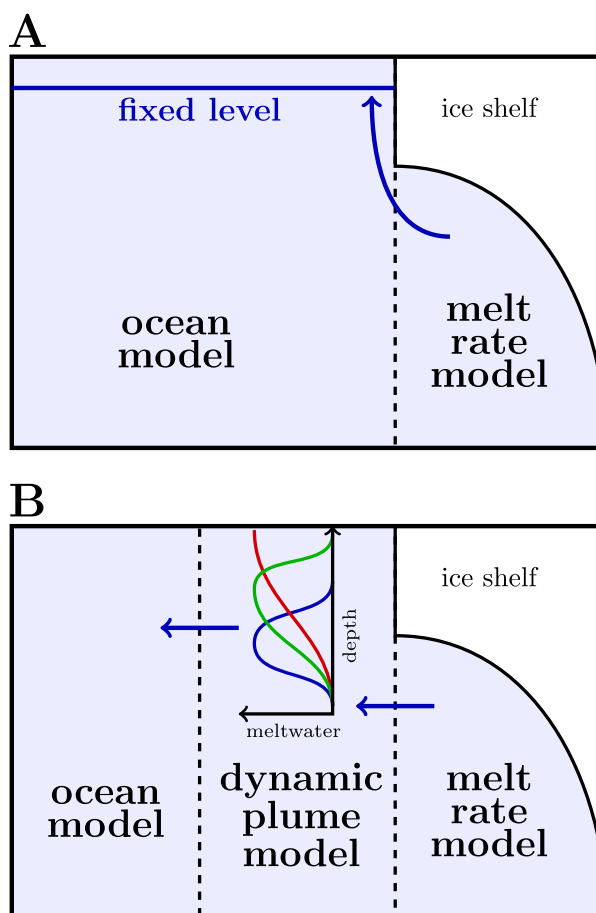
FIG. 8. Schematic describing two different paradigms for Antarctic meltwater fluxes in simulations of global climate. In paradigm A, the fluxes from a melt rate model are inserted into the ocean model at some fixed vertical level; this approach has dominated the literature. In paradigm B, the melt rate model is coupled to a dynamic plume model that describes the small-scale dynamics of buoyant meltwater plumes and accurately calculates the vertical distribution of meltwater for insertion into the ocean model. Given the potential climatic importance of glacial meltwater, the strong dependence of settling depth on the buoyancy forcing, and the vast heterogeneity in the observed mass loss rates and ambient conditions at different ice shelves, this approach would likely represent a significant improvement over the one-size-fits-all approach of paradigm A.
