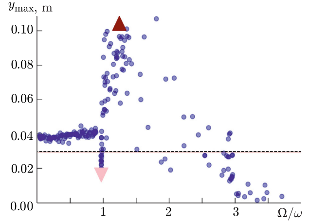
Fig. 3. Bridge amplitude y_{\max} after the time t = 30 s as a function of 200 different combinations of bridge and pedestrian natural frequencies \Omega_0 and \omega_1 , yielding frequency ratios \Omega/\omega . Here, \Omega and \omega are the numerically calculated bridge and pedestrian frequencies whose ratio corresponds to different combinations of \Omega_0 and \omega_1 (blue points). The dashed horizontal line represents the initial level of bridge oscillations with y(0) = 0.03 m and \dot{y} = 0.001 m/s. The thin red line corresponds to final y_{\max} = 0.0297 after t = 30 in the absence of the pedestrian motion. The points above the red line indicate amplified pedestrian-induced bridge oscillations. The points below the red line yield combinations of \Omega and \omega for which the pedestrian damps the bridge oscillations. The points indicated by the red and pink triangles correspond to the maximum and minimum values of the amplitude resonance curve near the 1 : 1 resonance. Other bridge parameters are M = 3000 kg and h = 0.001 N s/m. Pedestrian parameters are as in Fig. 2, except for varying \omega_1 . The integration step varies with an upper bound of 0.001.
