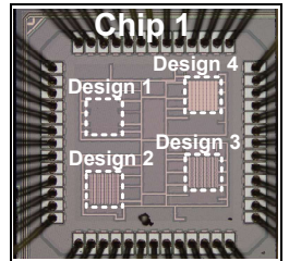
Fig. 7 Chip-1 die photo showing 4 AES cores
