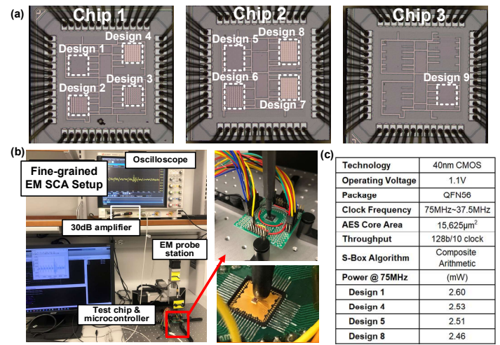
Fig. 4. (a) Die photos of Chip 1: power grid designs, Chip 2: Decap cells with VSS shield designs, and Chip-3: isolated S-Box placement design (b) Fine-grained EM SCA setup, closeup photo of the EM probe with the packaged and de-packaged chip (c) AES core design parameters and measured power consumption
