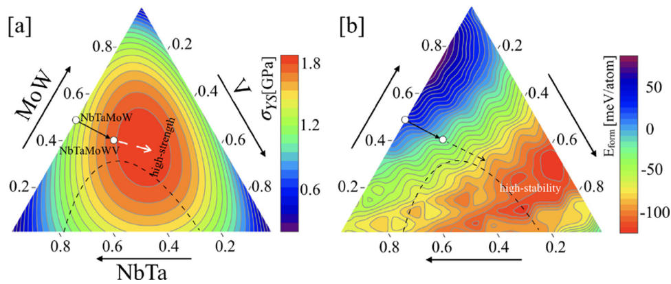
Fig. 7. (a) Yield-strength ( \sigma_{oy} ) and (b) formation enthalpy ( \Delta H_{form} at 0 K) vs composition ( c_i , i =Nb/Ta, Mo/W, V). The parabolic-dashed line shows the high electronegativity variance ( \Delta\chi_{var} ), while arrow-head from NbTaMoW to NbTaMoWV RHEA (solid-white circle) shows experimentally observed increasing trend. Our observation suggests that its not the single parameter but the interplay of different quantities, such as chemical entropy, \Delta\chi_{var} , and \Delta H_{form} , that are responsible for higher strength.
