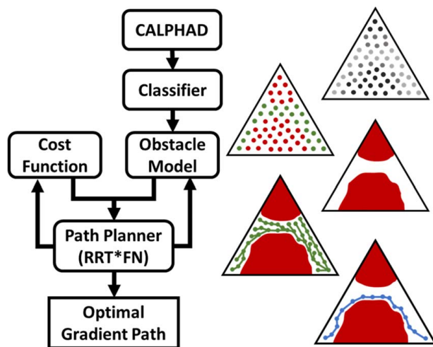
Fig. 1 Computational FGM design methodology presented in Ref. [18]. CALPHAD data are used to train machine learning classifiers that model the obstacles in the state space. These obstacle models and a user-defined cost function are sampled by the path planner (RRT*FN) to find the optimal gradient path through the state space.
