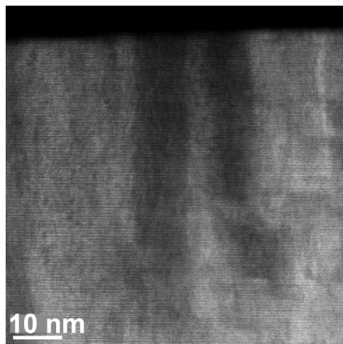
FIG. 9. STEM-HAADF image of \text{In}_{0.25}\text{Ga}_{0.75}\text{N} film grown on GaN at 560 °C.
