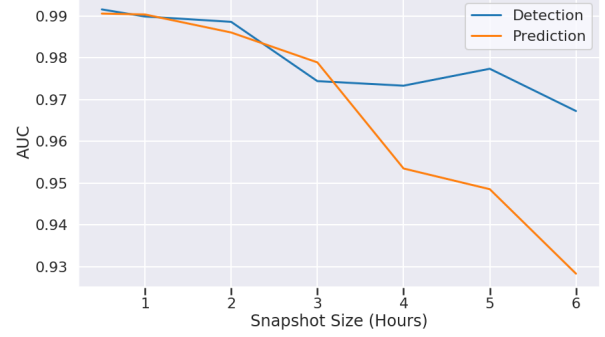
Fig. 4: Change in AUC score as \delta increases for link prediction and detection with GCN+GRU models. Scores are the average of five tests on the LANL dataset.
