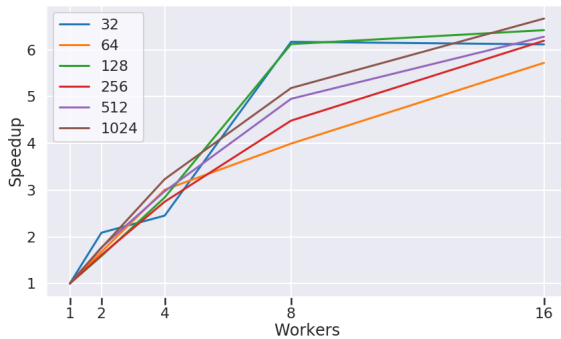
Fig. 6: Performance improvements as more workers are added for varying numbers of snapshots from the LANL data set. The model used was a GCN stacked on a GRU. All time windows, \delta are 0.5 hours.
