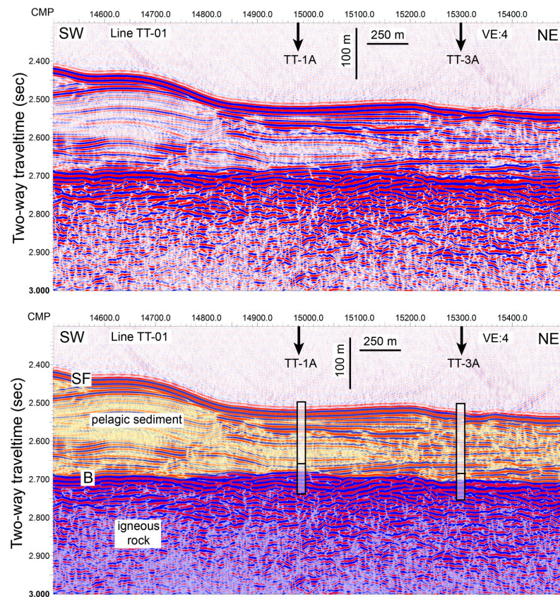
Figure F5. Seismic profile crossing proposed Site TT-3A. Top: uninterpreted data. Bottom: interpretation. Site TT-1A is located on another seismic line and is slightly off this line (see Figure F3). Columns = approximate intervals to be drilled, horizontal line in column = approximate depth at which coring will begin. CMP = common midpoint, VE = vertical exaggeration. SF = seafloor, B = acoustic basement.
