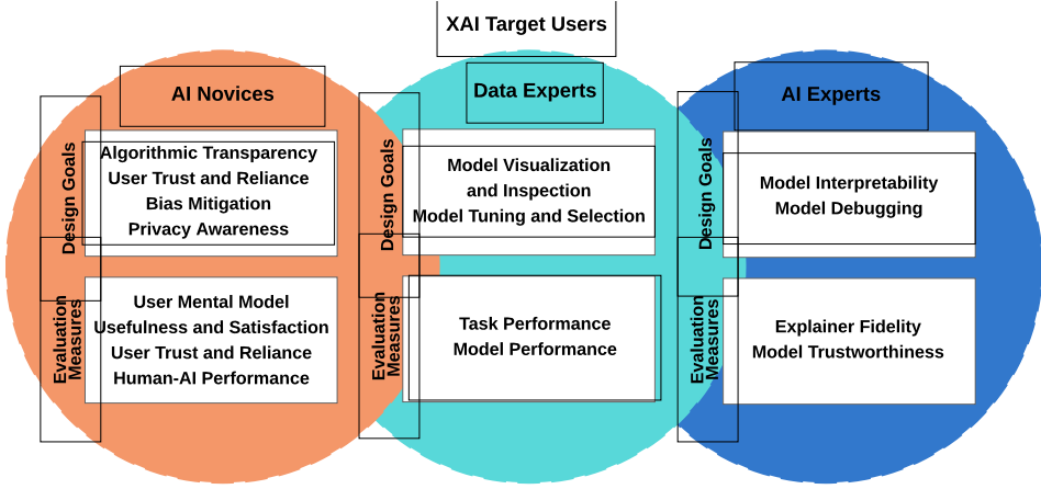
Fig. 3. A summary of our categorization of XAI design goals and evaluation measures between user groups. Top: Different system design goals for each user group. Bottom: Common evaluation measures used in each user group. Notice that similar XAI goals for different user groups require different research objectives, design methods, and implementation paths.
