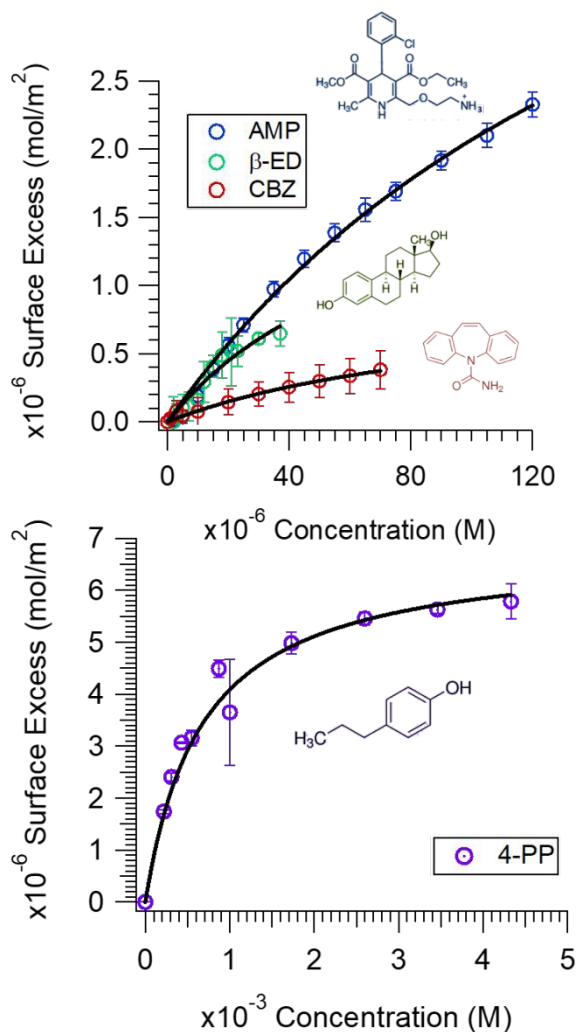
Figure 1 Adsorption isotherms (surface excess vs. initial concentration) of AMP, \beta -ED, CBZ (Top) and 4-PP (Bottom) for the air/aqueous interface. The solid black traces correspond to the Langmuir fits of the experimental data. Images of molecular structures are from Sigma Aldrich.
