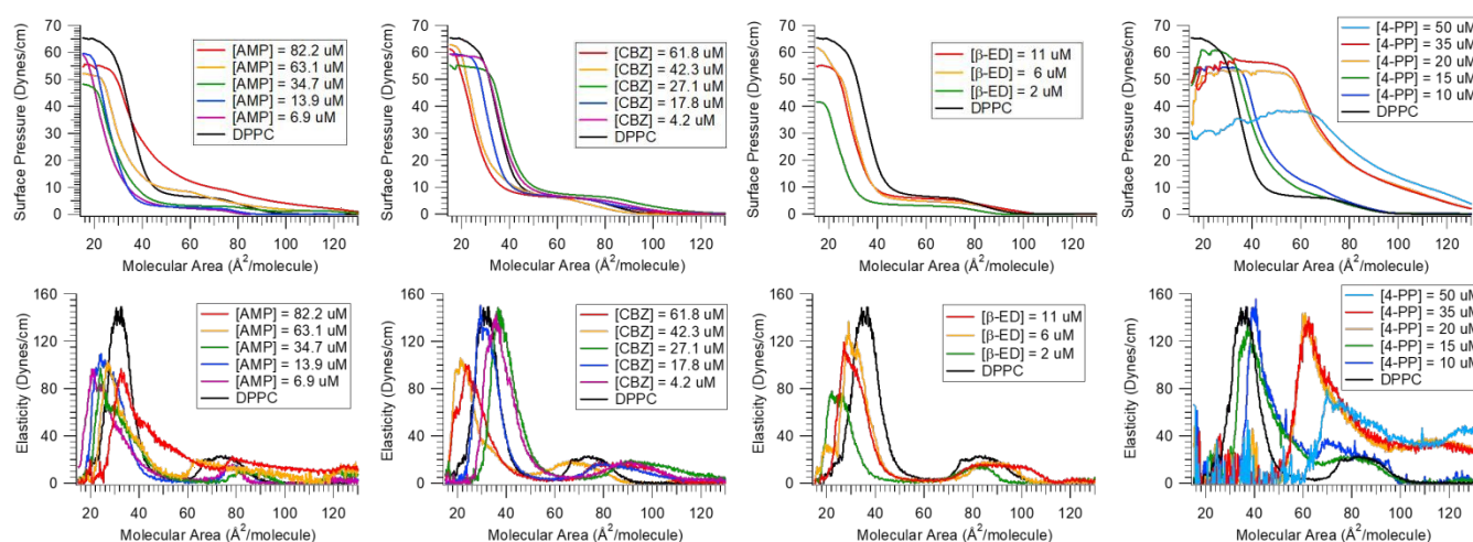
Figure 2 Surface pressure vs. molecular area isotherms and elasticity vs. molecular area plots of DPPC in the presence of micropollutants, from left to right: AMP, CBZ, \beta -ED, and 4-PP. The concentration of the contaminant in the sub-phase is noted in the legend. The black trace is the measurement corresponding to DPPC in the absence of any micropollutant (i.e., neat water sub-phase).
