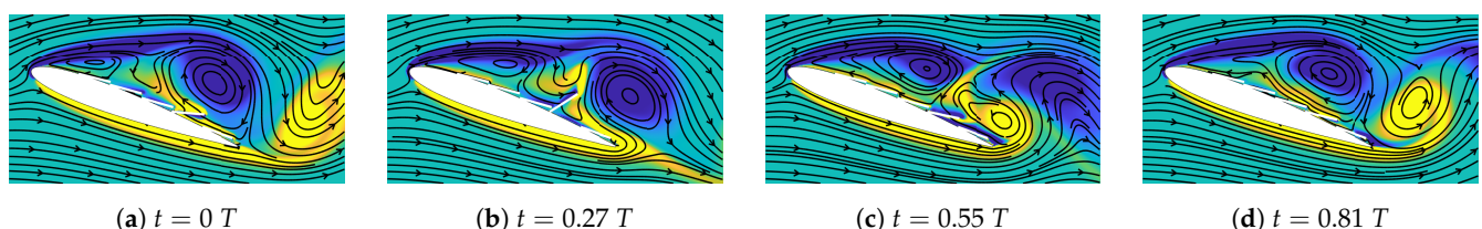
Figure 9. Vorticity contours at different time instants in one period of lift cycle for the case of k_\beta = 0.005 and i_\beta = 10^{-5} .
