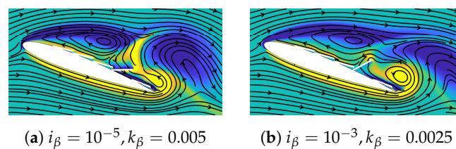
Figure 11. Vorticity contours at t/T = 0.45 demonstrating the downward-moving flap 4 countering the TEV and its reverse flow.
