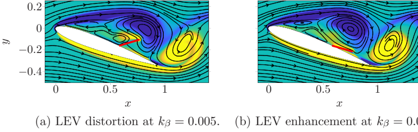
FIG. 21. Demonstration of LEV deformation as it advects above the flap at t/T = 0.82 for m_\beta = 1.875 and 60% chord via vorticity contours.
