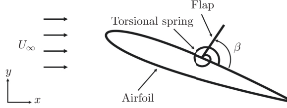
FIG. 1. Schematic of the system of a passively deployable flap on an airfoil.
