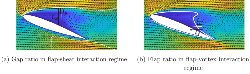
FIG. 30. Demonstration of length scales in the primary flow regimes. Both contour plots are identical and correspond to the mean velocity magnitude of the flap-less case.
