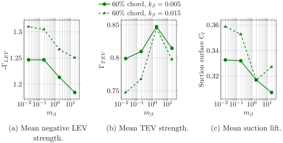
FIG. 27. Plots of various physical quantities characteristic of varying inertia in the flap-vortex interaction regime averaged over one time period for 60% location, and varying mass ratio and stiffness.
