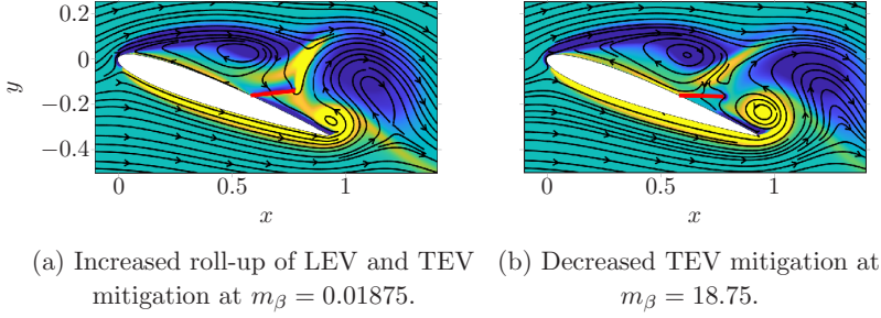
FIG. 26. Demonstration of the mitigation of TEV and roll-up enhancement of LEV facilitated by the downward-oscillating flap via vorticity contours with superimposed streamlines at t/T = 0.45 for k_\beta = 0.015 and 60% chord.
