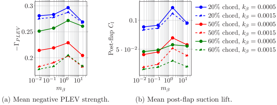
FIG. 19. Plots of various physical quantities characteristic of varying inertia in the flap-shear interaction regime averaged or integrated over the LEV-dominant portion of the lift cycle for different locations, mass ratios and stiffness.
