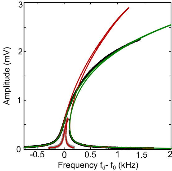
FIG. 2. Duffing response and non-Duffing response. Measured nonlinear response curves at drive voltages of V_d = 9 (gray) and 40 mV (black). Both traces display unprocessed raw data; the noise level remains below the size of the dots. A fit to the Duffing model at V_d = 9 mV as well as a theory curve using the obtained \gamma_{\text{eff}}^{(V)}/(2\pi)^2 = 2.48 \times 10^{15} \text{ V}^{-2} \text{ s}^{-2} for V_d = 40 mV are included (red lines). The deviation of the data from the Duffing model is clearly visible for the V_d = 40 mV data. A better agreement is achieved by taking the influence of the cubic nonlinearity of the potential \beta into account (green line). The curve is calculated for \beta^{(V)}/(2\pi)^2 = 2.08 \times 10^{15} \text{ V}^{-1} \text{ s}^{-2} and is truncated at a detuning of 2 kHz.
