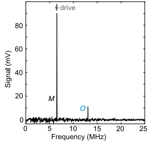
FIG. 3. Spectrum of the resonantly driven fundamental mode ( M ). For a resonant drive at f_d = f_0 = 6.528 MHz with V_d = 100 mV, the overtone ( O ) at 13.056 MHz is clearly visible. Higher-order overtones are barely discerned in this representation. A constant noise background has been subtracted from the data.
