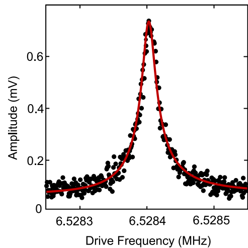
FIG. 7. Linear response of the fundamental out-of-plane mode ( M ) at a drive voltage of V_d = 1 mV. A Lorentzian fit (red line) yields an eigenfrequency of 6.528 MHz, a linewidth of 2\Gamma/(2\pi) = 20 Hz, and a quality factor of Q \approx 325\,000 .
