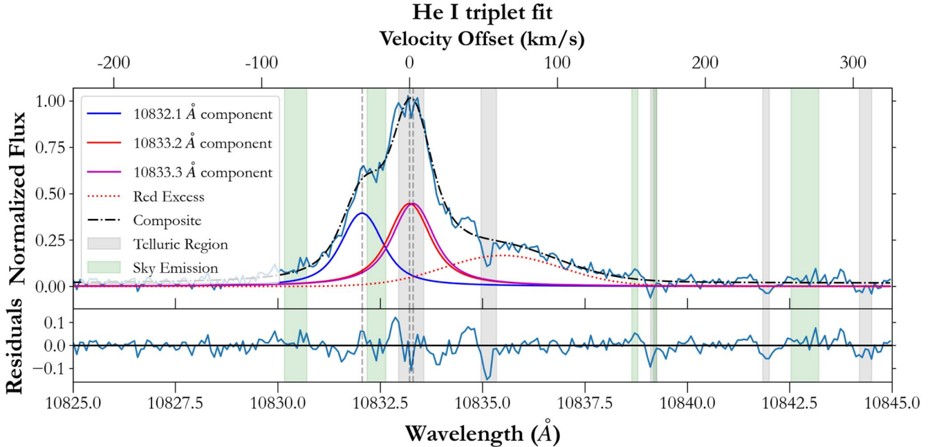
Figure 7. Voigt fit to the He triplet emission for T1 (Figure 5), showing the three components, as well as excess emission at the red wing of the triplet ( \sim 10836 Å). The rest wavelength for each line is marked with a dashed line. The shaded gray regions indicate where the telluric model (Section A.1) shows >10\% telluric absorption (before correction) and are masked while fitting the line profiles. Similarly, the green regions mark the sky emission lines. We also fit the red excess with a Gaussian and find the peak of the red components at about ( 10835.5 Å). The red excess seen here is about 30% in magnitude of the total He I triplet emission.
