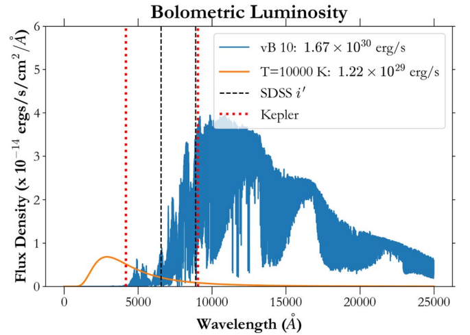
Figure 10. In this plot we show a BT-Settl model spectrum (Allard et al. 2012) at 2700 K for vB 10, in addition to a scaled 10,000 K blackbody. The black dashed line indicates the SDSS i' bandpass used for the observations in Section 4 to estimate the continuum enhancement, while the red dotted line shows the Kepler bandpass used for the analysis in Section 6.3. The bolometric luminosity for vB 10 is 1.67 \times 10^{30} erg s ^{-1} (Tinney et al. 1993), while that for the 10,000 K blackbody is 1.22 \times 10^{29} erg s ^{-1} . This suggests that right before the HPF observations the bolometric luminosity of the flare was \sim 7\% of the total luminosity of the star.
