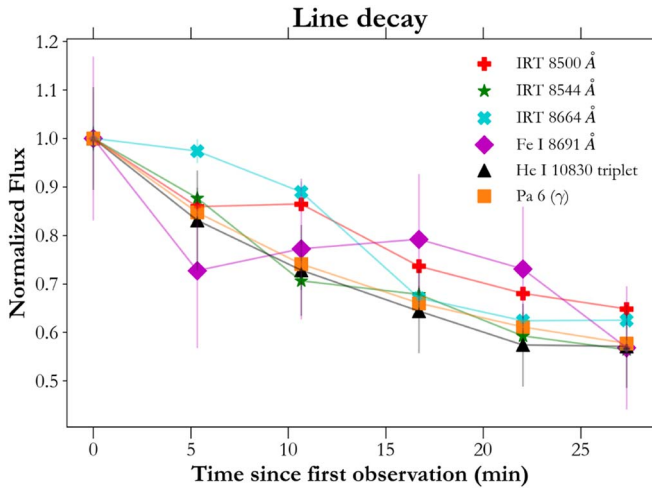
Figure 9. We split the 945 s HPF NDR exposure into three subexposures of 315 s each. For each of the lines, we show the normalized fluxes for the six HPF exposures as a function of exposure midpoint. We fit a linear decay to the 315 s fluxes, the average slope of which is about -1.5\% minute ^{-1} . The fluxes for the NDR exposures are calculated by summing across a 2 Å window for the calcium and iron lines and a 5 Å window for the Paschen lines and helium triplet. The window is narrow enough that the relative change in the instrument response across that window is negligible, and hence the error bars depicted in this plot are based on the propagated variance for each line.
