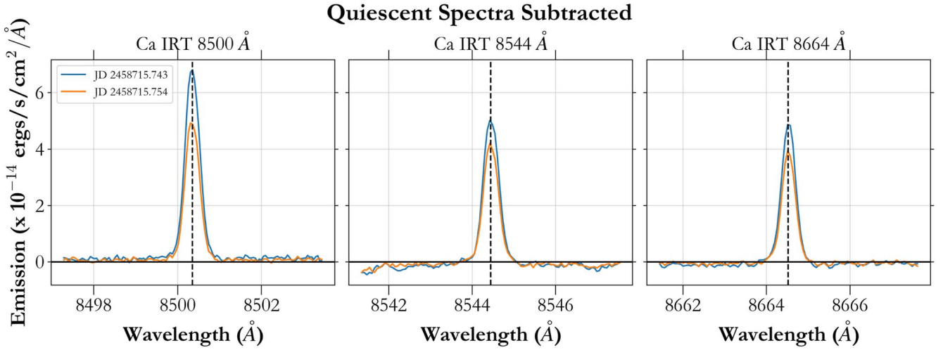
Figure 2. Quiescent-subtracted spectrum from HPF showing the emission in the Ca IRT seen in vB 10. The dashed lines mark the rest position of each line. The two different colors indicate the successive HPF observations.
