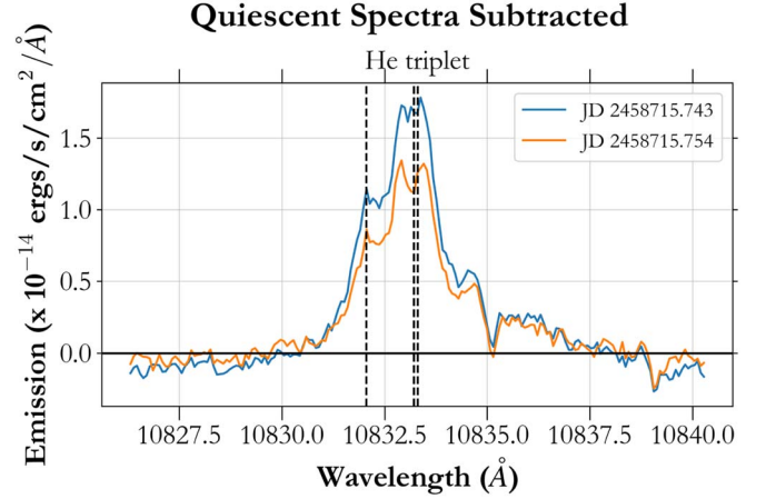
Figure 5. Quiescent-subtracted spectrum from HPF showing the He triplet lines seen in emission in vB 10. The dashed lines mark the rest position of each line. The two different colors indicate the successive HPF observations. The triplet is one of the strongest emission features we see in the HPF spectra and is consistent with being optically thick.
