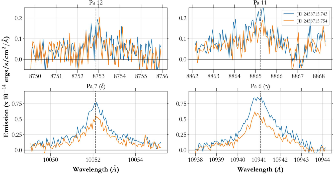
Figure 3. Quiescent-subtracted spectrum from HPF showing the Pa lines seen in emission in vB 10. The dashed lines mark the rest position of each line. Blue and orange depict the two observations—T1 and T2, respectively.
