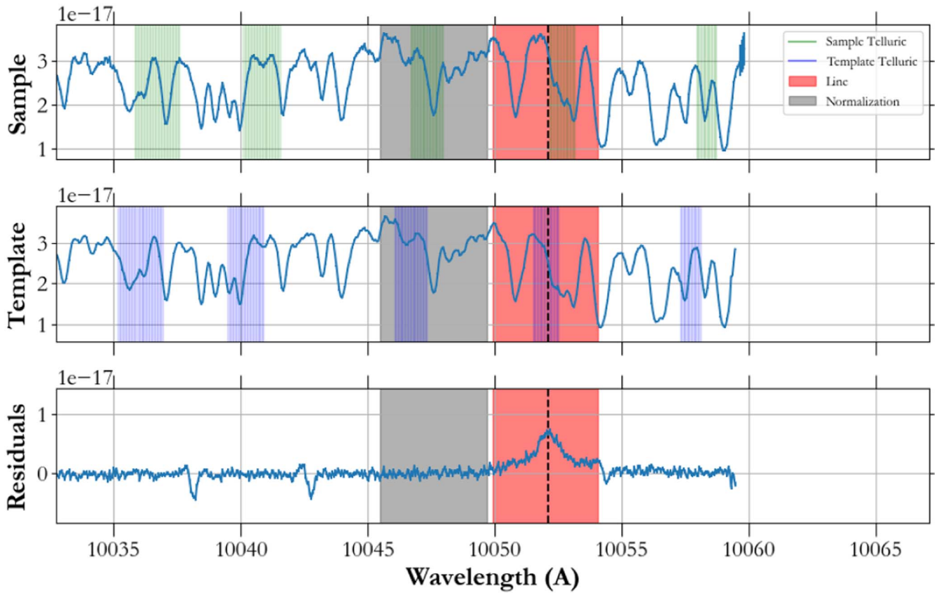
Figure 13. An example of the spectral subtraction, with the sample spectrum shown in the top panel, the template in the middle panel, and the residuals in the bottom panel. While the excess at the position of the Pa 7 ( \delta ) line is apparent in the residual spectrum, it is harder to tease out before subtracting a quiescent template.
