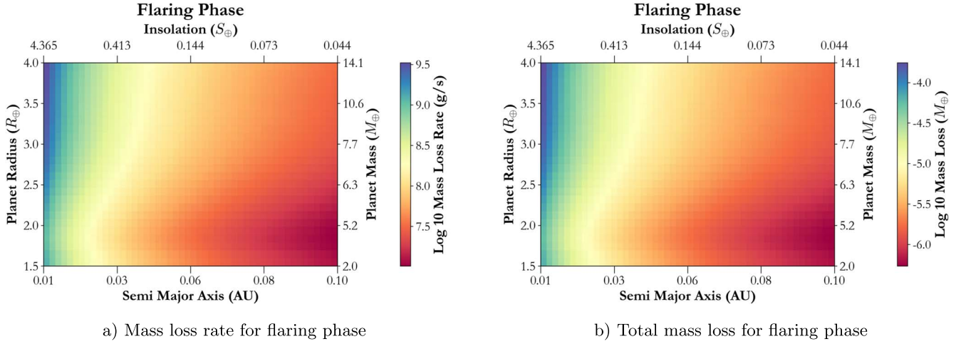
Figure 11. The atmospheric mass loss across a range of small planet radii ( 1.5\text{--}4 R_{\oplus} ), and semimajor axis spanning 0.01\text{--}0.1 au using Equation (1). (a) The rate of mass loss, assuming a high-energy luminosity ( L_{\text{HE}} = 10^{27} \text{ erg s}^{-1} ) equivalent to Fleming et al. (2000). To calculate the insolation at different separations for vB 10, we use the bolometric luminosity of \log L_{\text{bol}} = -3.36 (Tinney et al. 1993). (b) We propagate the mass-loss rate over 1 Gyr to calculate the cumulative atmospheric mass loss for a small planet around vB 10, with a flare duration of 1 hr and frequency of once per 100 hr, as estimated in Section 6.3. As discussed in Section 6.4, the mass loss during the quiescent phases should be approximately double the loss from such flares. The relatively low mass-loss rate estimated for vB 10 is consistent with its low v \sin i and is likely to have been higher earlier in its lifetime.
