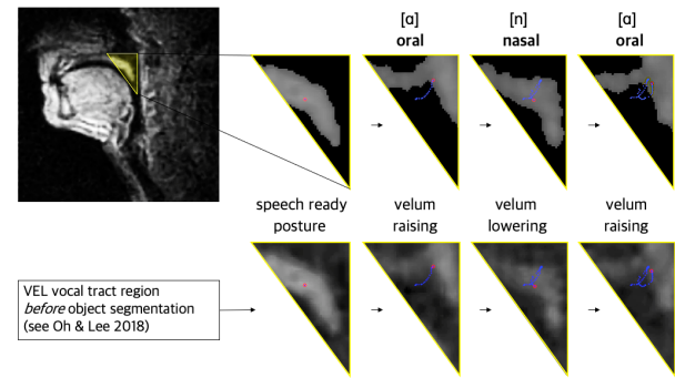
Figure 1: Velum centroid tracking example for [ana].
