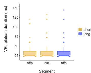
Figure 6: Velum plateau duration.
