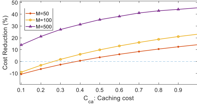
Fig. 6: Average cost reduction per edge cache by K = 3 distributed caching with \alpha = 1 .
