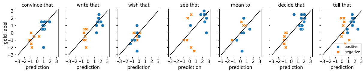
Figure 3: Multi model's predictions compared to gold labels for certain verbs and frames in RP. Diagonal line shows perfect prediction.
