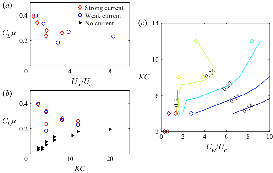
Figure 4. Drag parameter C_D \alpha versus ratio of wave orbital velocity to current in the canopy layer ( U_w/U_c ) and Keulegan–Carpenter number ( KC ). In (a,b), red diamonds are simulations with strong current (cases 6–10), blue circles are simulations with weak current (cases 1–5), and black triangles are simulations with no current from Yu et al. (2018). In (c), diamonds are strong current cases, circles are weak current cases, and lines are contours of C_D \alpha ; points and contours are coloured according to C_D \alpha .
