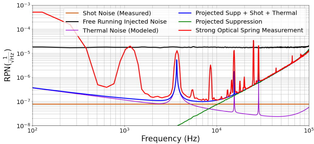
Fig. 3. 70 \mu W power noise spectrum post cavity measurement with its associated fundamental noise limitations, which includes relative shot noise, the calculated (modeled) RPN, and projected suppression of the cavity. The circulating power corresponding to 70 \mu W of transmitted power is 250 mW.
