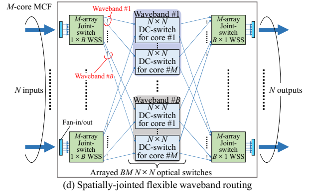
Fig. 2 N \times N OXC node configurations.
