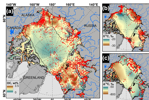
Figure 2. CASCADE data location for OC concentrations (a). Carbon isotopes \delta^{13}\text{C} (b) and \Delta^{14}\text{C} (c) marked as red dots, with interpolated fields as indicated by the inserted color scale and as described in the main text.
