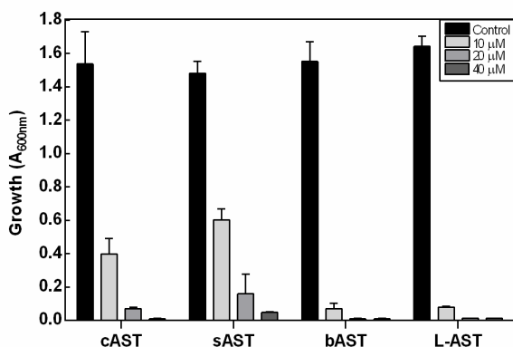
Figure 1. AST inhibits growth of E. coli . Cells were cultured in M9 medium in the absence or presence of the indicated concentrations of D/L-cAST, D/L-sAST, L-bAST, L-AST. Growth was estimated from the A 600nm after 16 h. Data are the mean ± SE (n = 3).
