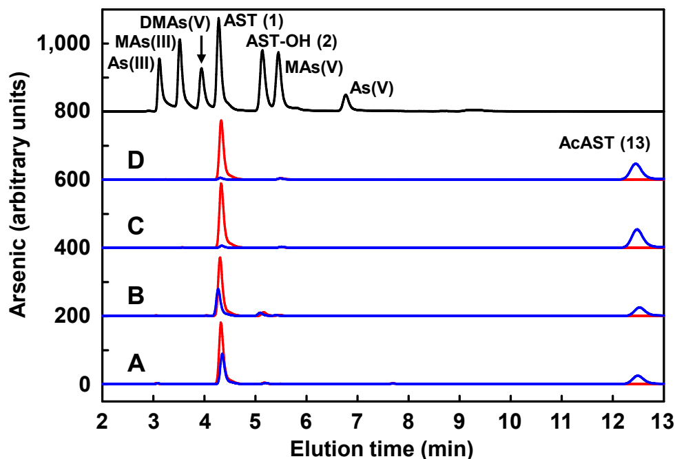
Figure 2. Enzymatic acetylation of 1 to produce 13 . Chemically synthesized D/L-cAST (A), semisynthetic D/L-sAST (B), biogenic L-bAST (C) or L-enantiomeric (D) 1 was incubated in the absence (red lines) or presence (blue lines) of PpArsN1. The arsenic species in the reaction solutions were analyzed by HPLC-ICP-MS. Abbreviations: As(III), arsenite; MAs(III), methylarsenite; DMAs(V), dimethylarsenate; AST ( 1 ), arsinothricin; AST-OH ( 2 ), hydroxyarsinothricin; MAs(V), methylarsenate; As(V), arsenate; AcAST ( 13 ), N -acetylarsinothricin.
