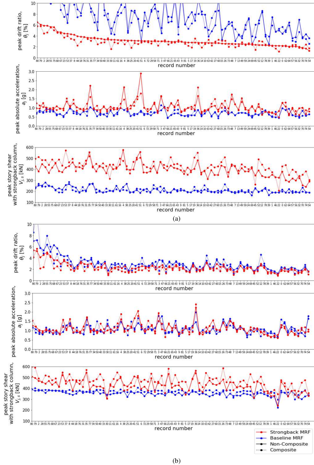
Fig. 8 – maximum of peak story drift ratio, absolute acceleration and story shear over all stories for: (a) pinned column bases and (b) fixed column bases.
