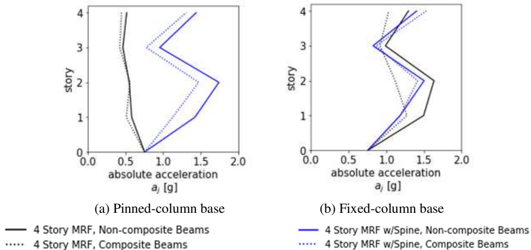
Fig. 6 – Peak absolute floor accelerations
