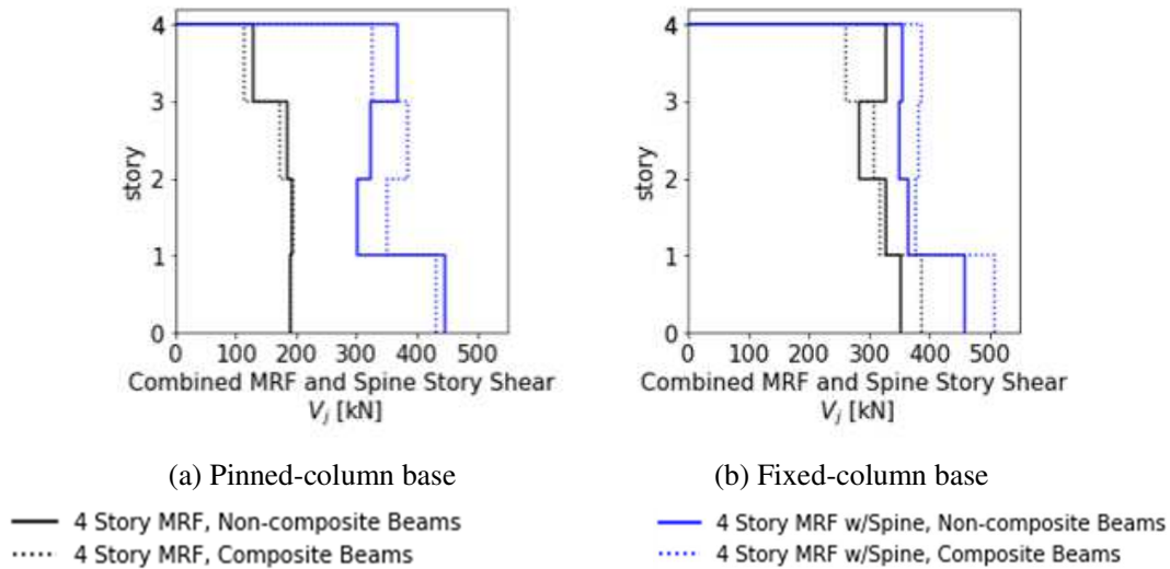
Fig. 5 – Peak story shear
