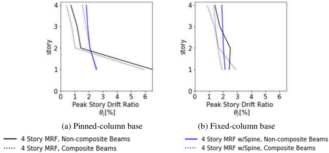
Fig. 4 – Peak story drift ratio
