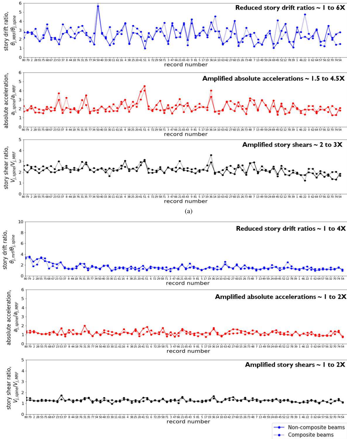
Fig. 9 – maximum of peak story drift ratio, absolute acceleration and story shear over all stories for: (a) pinned column bases and (b) fixed column bases.
