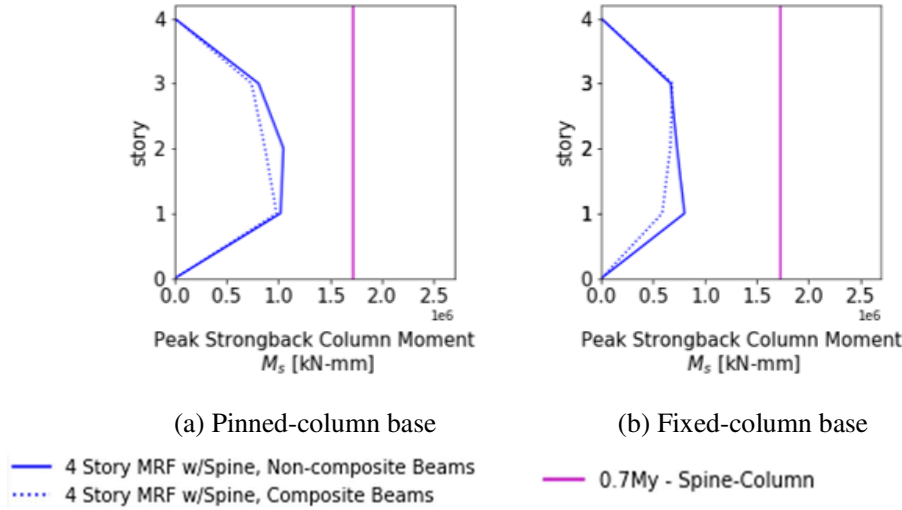
Fig. 7 – Peak moments in spine
