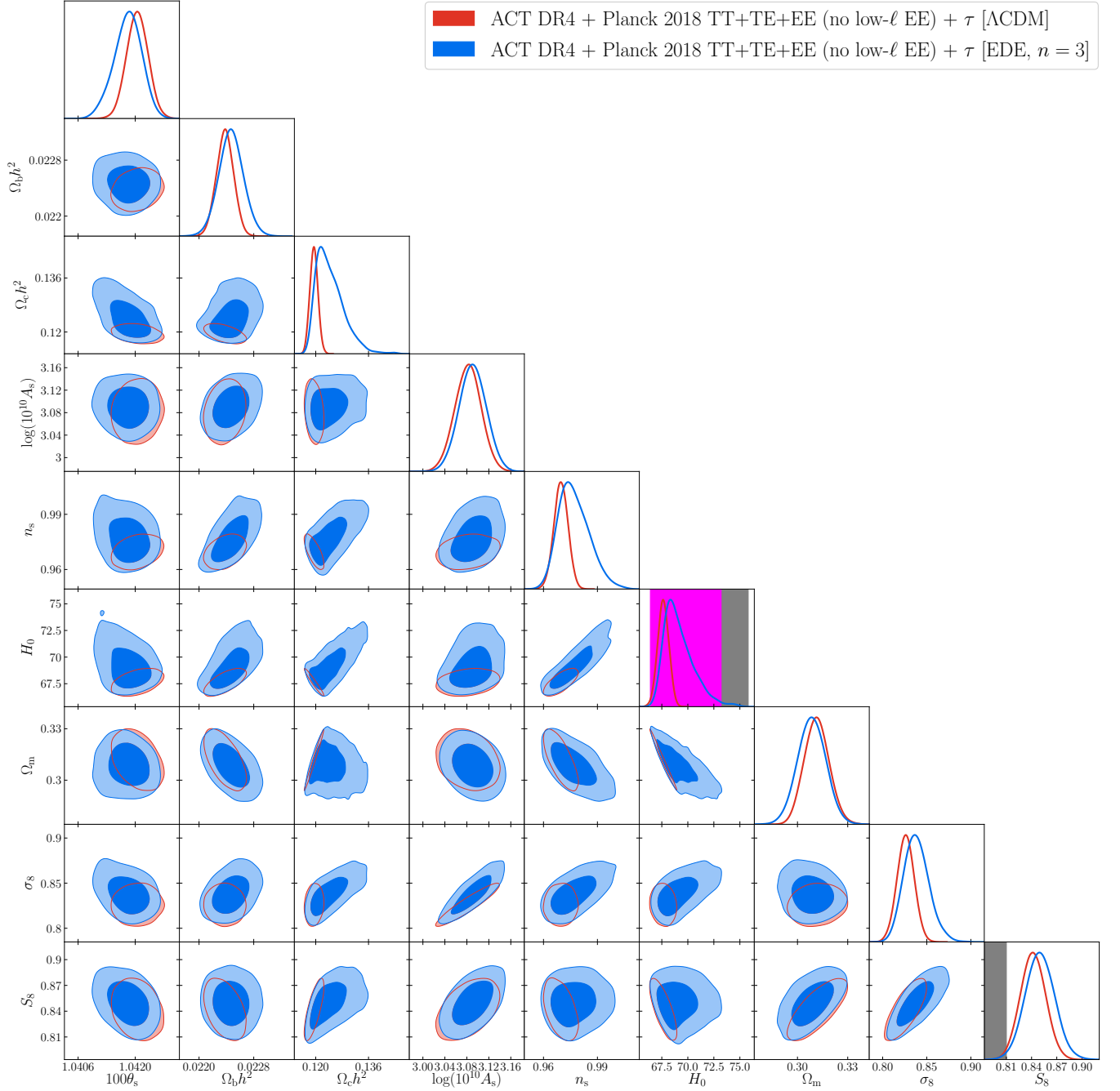
FIG. 17: Marginalized posteriors for the standard cosmological parameters in the \Lambda CDM (red) and EDE (blue) models fit to ACT DR4 TT+TE+EE and Planck 2018 TT+TE+EE (full \ell range, but no low- \ell EE) data in combination with a Gaussian prior on \tau , as presented in Sec. IV E . The vertical grey and magenta bands in the H_0 panel show the latest SH0ES [10] and TRGB [12] constraints, respectively. The vertical grey band in the S_8 panel shows the DES-Y3 constraint [73] .
