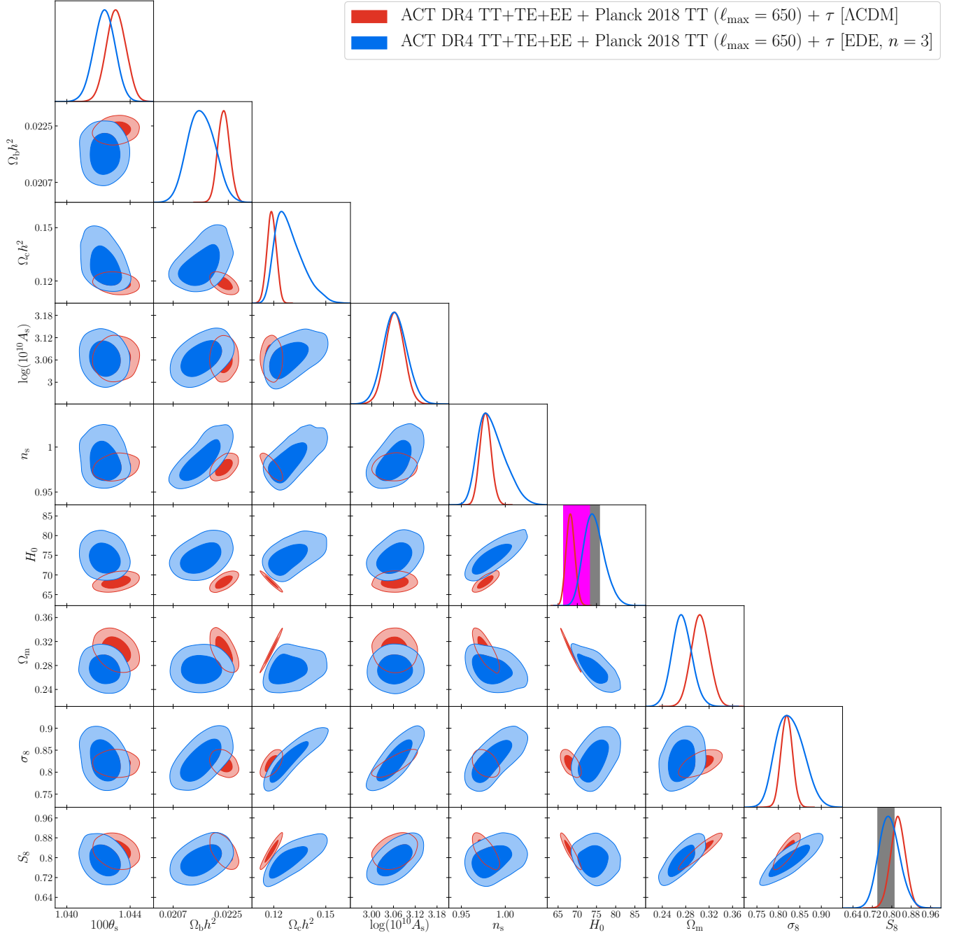
FIG. 14: Marginalized posteriors for the standard cosmological parameters in the \Lambda CDM (red) and EDE (blue) models fit to ACT DR4 TT+TE+EE and Planck 2018 TT ( \ell_{\text{max}} = 650 ) data in combination with a Gaussian prior on \tau , as presented in Sec. IV C . The vertical grey and magenta bands in the H_0 panel show the latest SH0ES [10] and TRGB [12] constraints, respectively. The vertical grey band in the S_8 panel shows the DES-Y3 constraint [73] .
