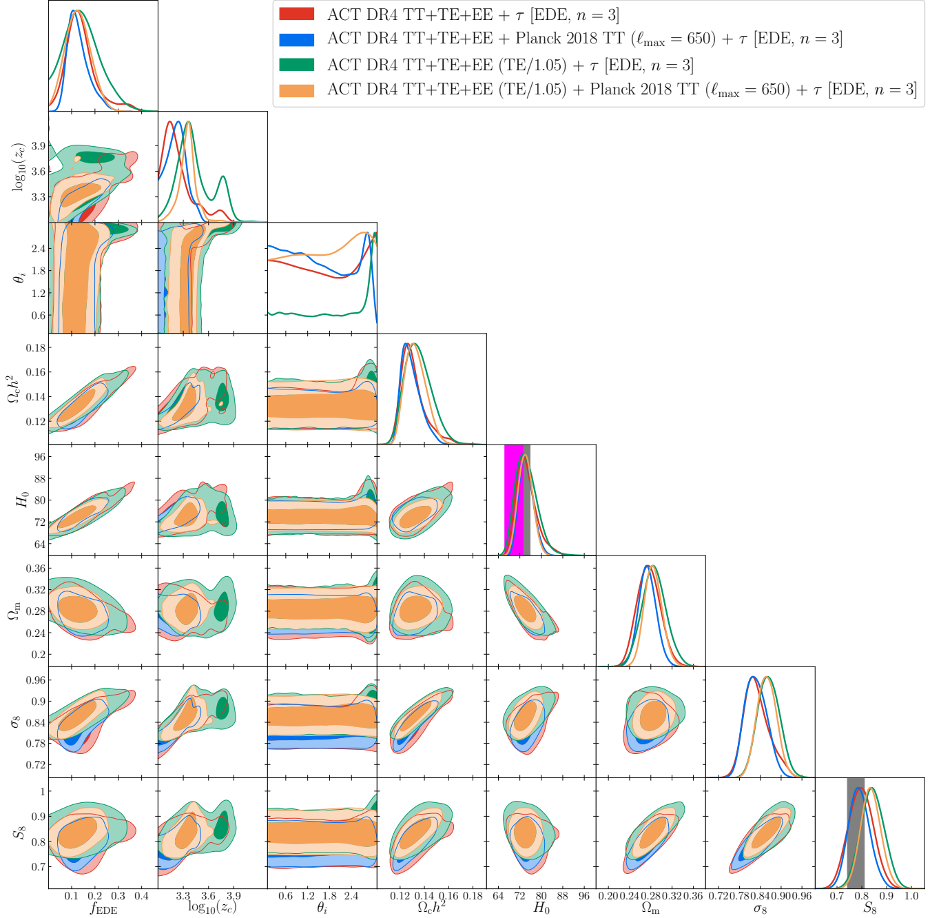
FIG. 18: Marginalized posteriors for the EDE parameters and a subset of other parameters of interest in fits to ACT DR4 TT+TE+EE (red) and ACT DR4 TT+TE+EE with Planck 2018 TT ( \ell_{\text{max}} = 650 ) (blue). The green and orange contours show results for the same data set combinations, but with the ACT TE data divided by 1.05. These results are discussed in Sec. IV B and IV C. The vertical grey and magenta bands in the H_0 panel show the latest SH0ES [10] and TRGB [12] constraints, respectively. The vertical grey band in the S_8 panel shows the DES-Y3 constraint [73].
