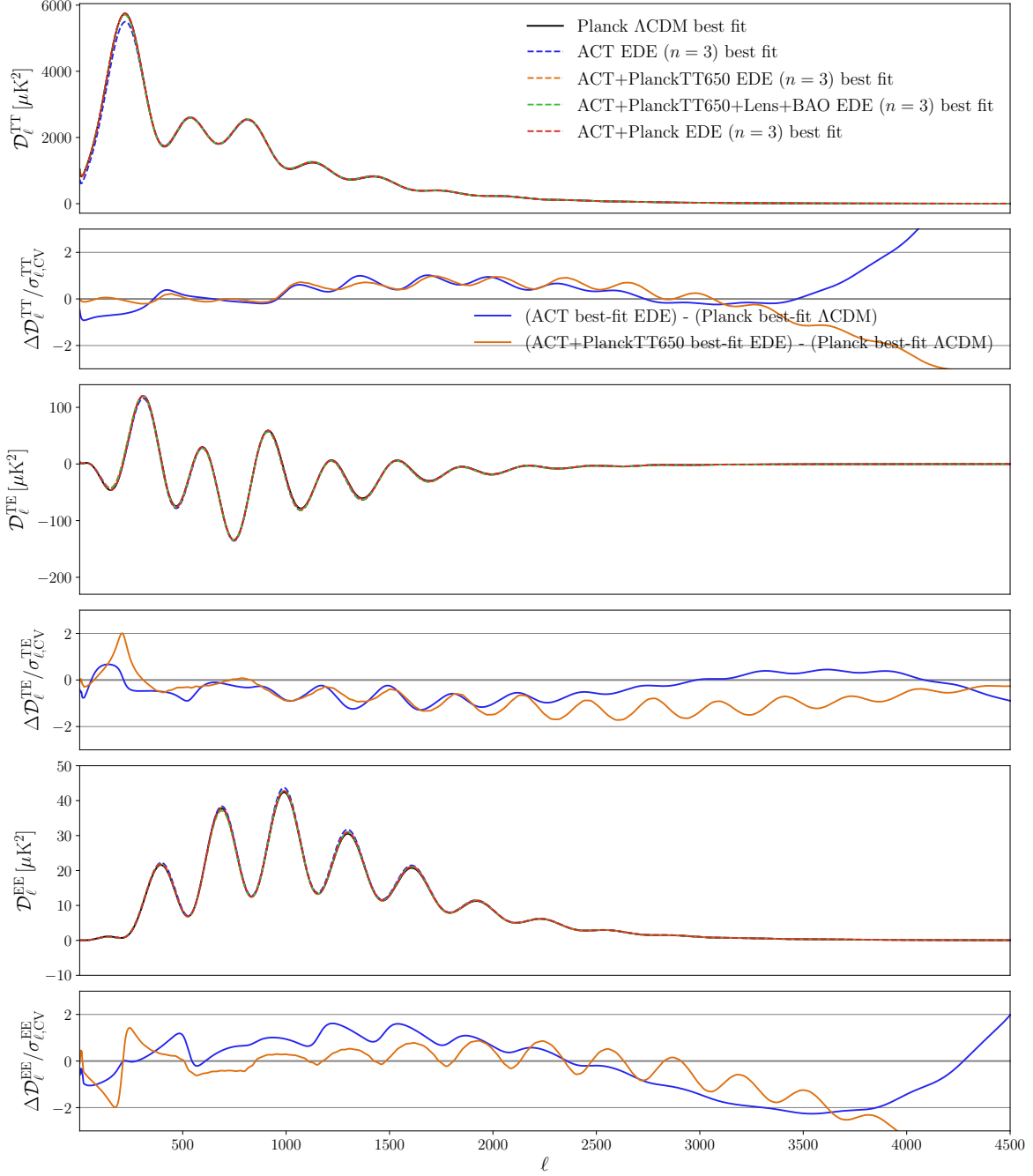
FIG. 25: Comparison of TT (top), TE (middle), and EE power spectra in the best-fit EDE models to the data set combinations considered in Sec. IV and the best-fit \Lambda CDM model to Planck data alone (the latter from Ref. [47], but in excellent agreement with Ref. [15]). The smaller panels show differences with respect to the Planck best-fit \Lambda CDM model in units of the CV-limited error bar at each \ell , with the \pm 2\sigma range demarcated by the thin grey lines. The blue curve shows residuals for the best-fit EDE model to ACT DR4 alone (Table II) and the orange curve shows residuals for the best-fit EDE model to ACT + large-scale Planck TT data (Table IV). The residuals shown here are similar to those seen with respect to the best-fit EDE model to Planck alone, shown in Fig. 7.
