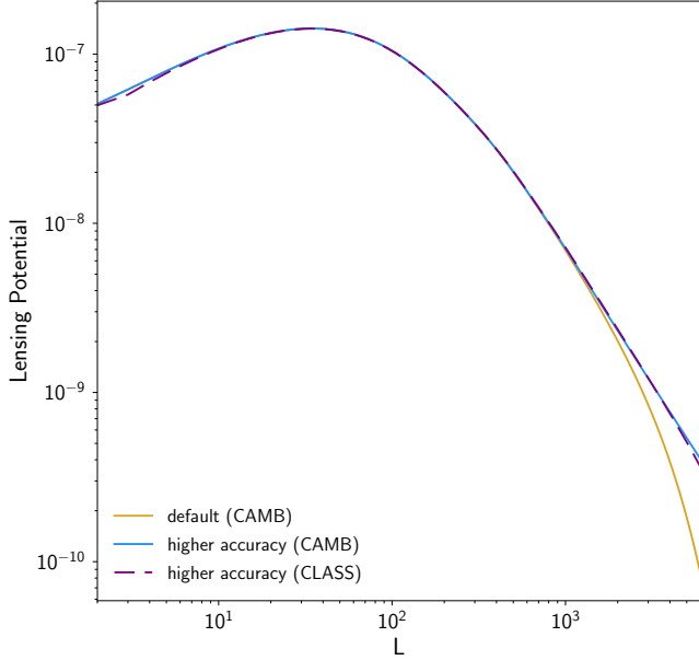
FIG. 8: CMB lensing potential power spectrum, [L(L+1)]^2 C_L^{\phi\phi}/(2\pi) , obtained with the CAMB default high-accuracy settings (solid orange), and with the higher-accuracy settings presented here from CAMB (solid blue) or CLASS (dashed purple). All curves are computed with identical cosmological parameters (column 4 of Table 4 in A20).
