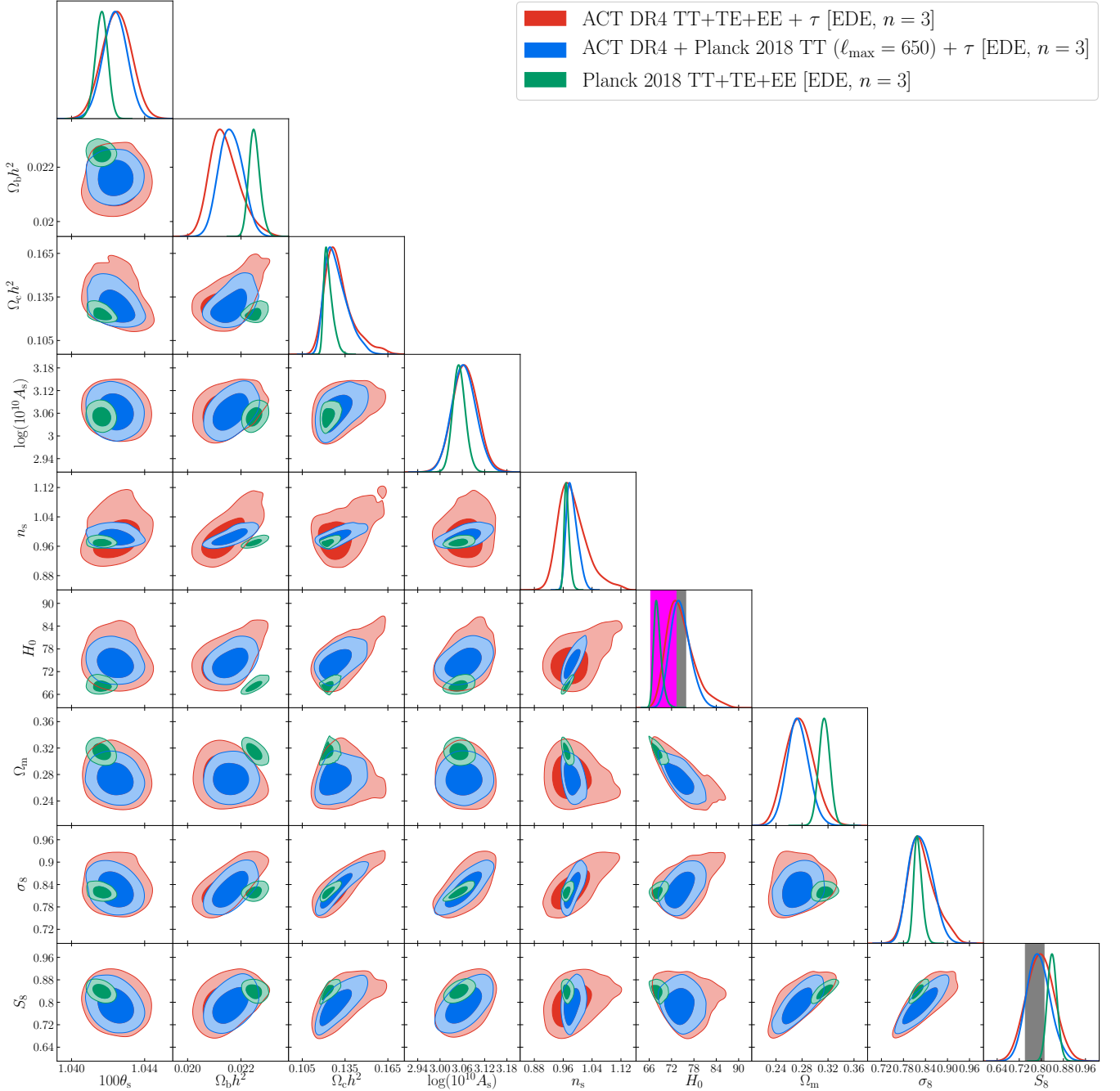
FIG. 15: Marginalized posteriors for the standard cosmological parameters in the EDE model fit to ACT DR4 TT+TE+EE data (red), ACT DR4 and Planck 2018 TT ( \ell_{\text{max}} = 650 ) data (blue), and Planck 2018 TT+TE+EE data (green, results from Ref. [47]). The vertical grey and magenta bands in the H_0 panel show the latest SH0ES [10] and TRGB [12] constraints, respectively. The vertical grey band in the S_8 panel shows the DES-Y3 constraint [73]. Within the EDE model, both ACT and ACT + large-scale Planck TT data appear to prefer somewhat different regions of parameter space than that preferred by the full Planck data set on its own, but the uncertainties in the ACT-based analyses are too large to draw strong conclusions at present.
