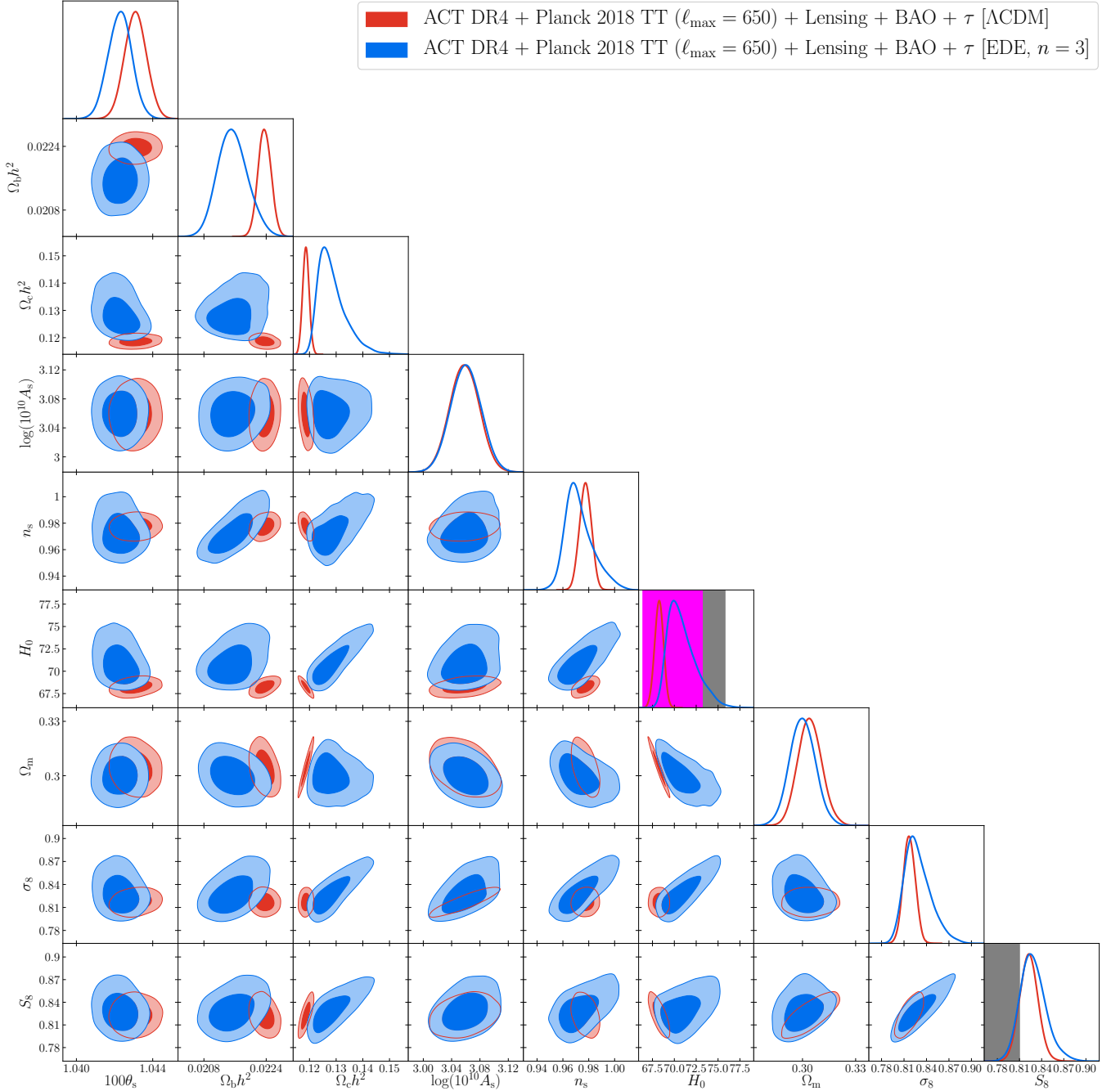
FIG. 16: Marginalized posteriors for the standard cosmological parameters in the \Lambda CDM (red) and EDE (blue) models fit to ACT DR4 TT+TE+EE, Planck 2018 TT ( \ell_{\text{max}} = 650 ), Planck 2018 CMB lensing, and BAO data in combination with a Gaussian prior on \tau , as presented in Sec. IV D. The vertical grey and magenta bands in the H_0 panel show the latest SH0ES [10] and TRGB [12] constraints, respectively. The vertical grey band in the S_8 panel shows the DES-Y3 constraint [73].
