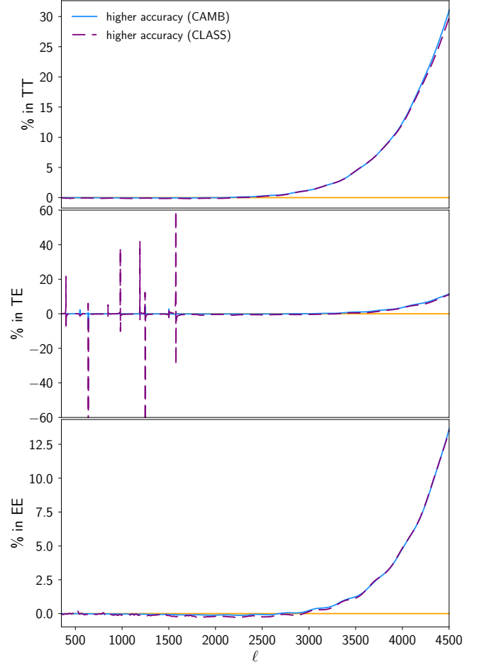
FIG. 9: Fractional differences in the lensed CMB TT, TE, and EE power spectra, (\text{higher-accuracy} - \text{default})/\text{default} , showing the deviation of the two sets of accuracy settings. The models and settings shown are identical to those used in Fig. 8.
