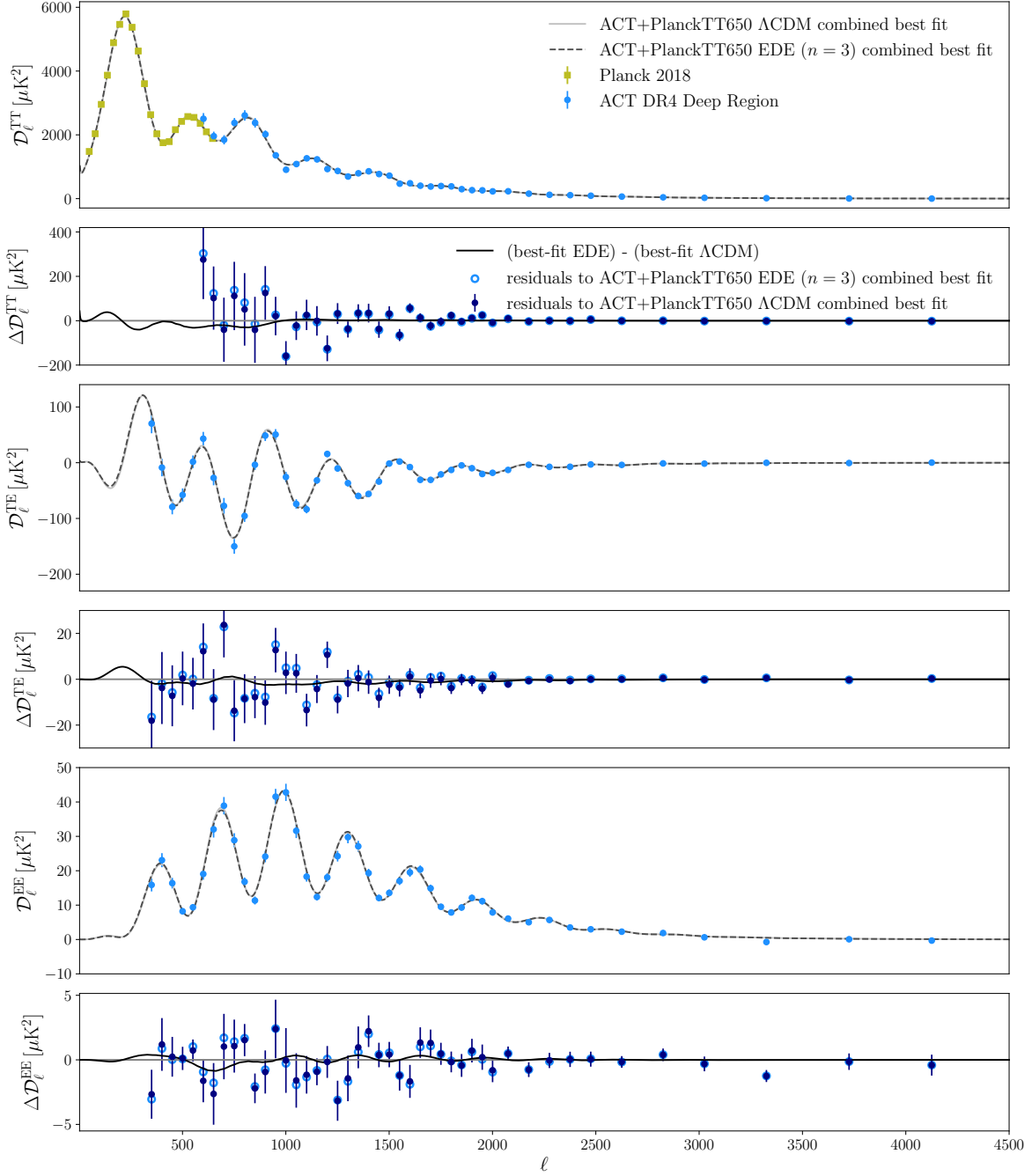
FIG. 24: Best-fit \Lambda CDM and EDE ( n=3 ) models to the ACT DR4 TT (top), TE (middle), and EE (bottom) power spectrum data, fit in combination with large-scale ( \ell_{\text{max}} = 650 ) Planck 2018 TT power spectrum data (yellow squares in top panel), shown here in comparison to the deep-patch ACT data. (The best-fit models are determined by the full data set shown in Fig. 4) The smaller panels show the residuals of the best-fit models with respect to the deep-patch data, as well as the difference between the best-fit EDE and \Lambda CDM models. The EDE \chi^2 improvement over \Lambda CDM (c.f. Table V) receives its largest contribution from the ACT deep-patch TE power spectrum shown here, although moderate improvements in TT and EE are also seen. The EDE- \Lambda CDM residuals in TE are distributed very evenly in \ell , with no individual bin differing by > 0.5\sigma .
