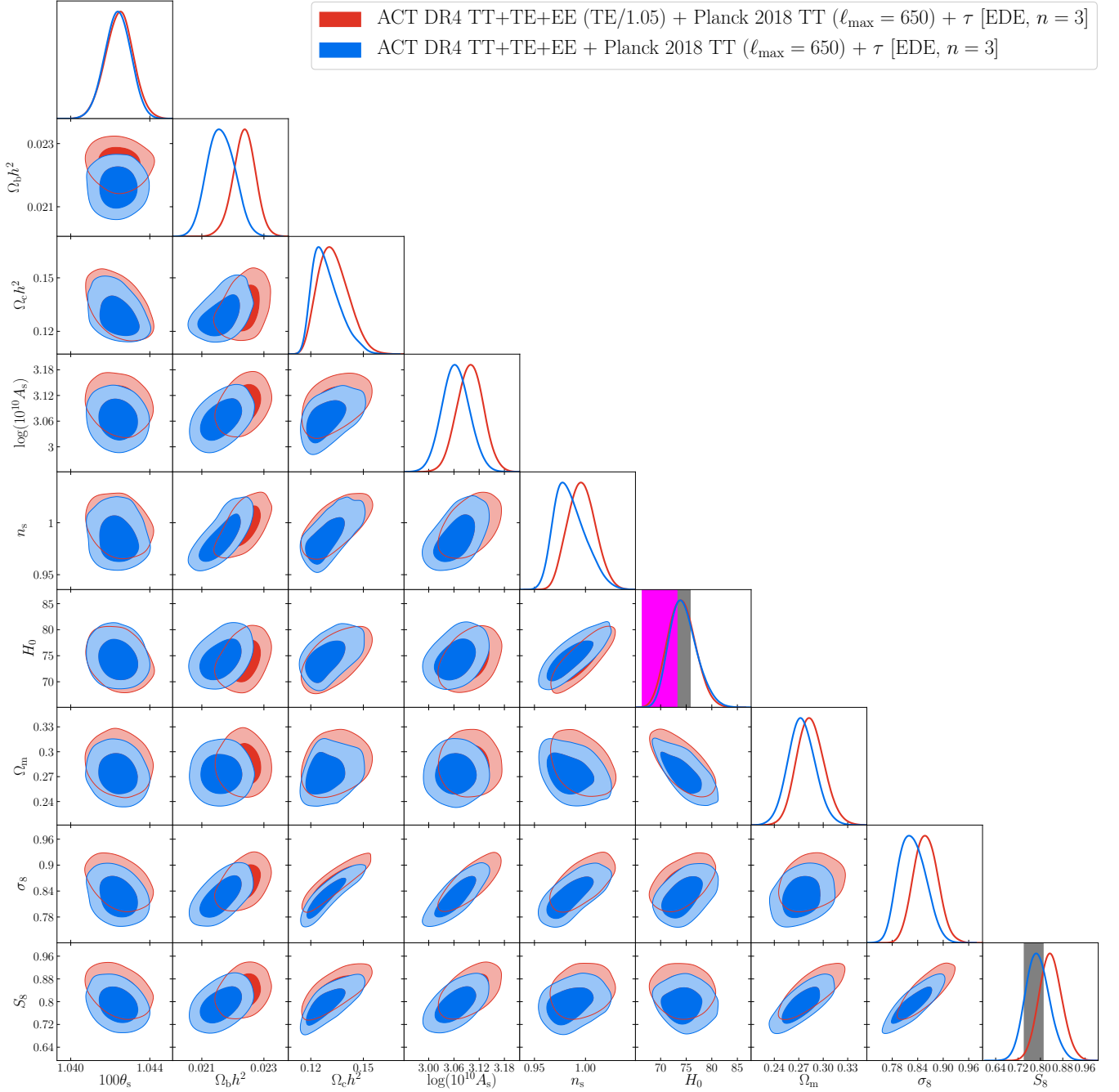
FIG. 20: Marginalized posteriors for the standard cosmological parameters in the EDE model fit to ACT DR4 TT+TE+EE and Planck 2018 TT ( \ell_{\text{max}} = 650 ) data in combination with a Gaussian prior on \tau , as presented in Sec. IV C. The blue contours show the results presented previously in Fig. 14, while the red contours show results found after dividing the ACT TE data by 1.05. The vertical grey and magenta bands in the H_0 panel show the latest SH0ES [10] and TRGB [12] constraints, respectively. The vertical grey band in the S_8 panel shows the DES-Y3 constraint [73].
