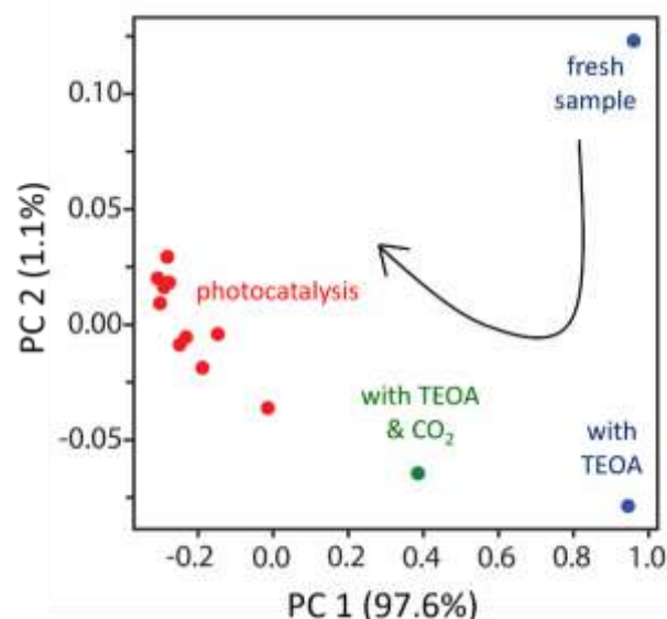
Figure 4. Plot of 1 st and 2 nd PCA components of each XANES spectra followed by a K-means clustering (different colours represent different clusters). PC 1 accounts for 97.6% of the total variation around all the spectra, and PC 2 accounts for 1.11%.
