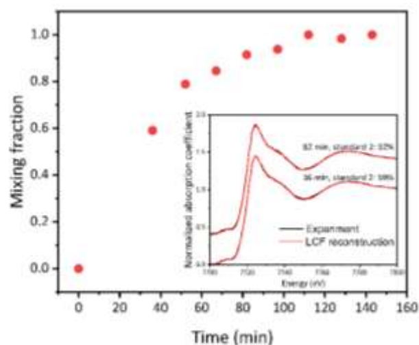
Figure 5. Linear combination fitting results showing the obtained mixing fraction of standard two. Standard one is the sample with TEOA and \text{CO}_2 purge before light. Standard two is the sample with light on for 143 min for reaction. Inset shows a comparison between the experimental XANES spectrum and the corresponding reconstruction of XANES spectrum from LCF result at 2 different reaction times.
