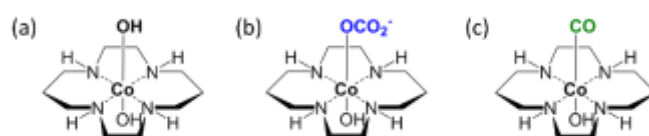
Figure 6. Proposed structures of Co(III) complex related to \text{CO}_2 reduction on Co-cyclam/ \text{C}_3\text{N}_4 , including the fresh sample(a), the sample with TEOA and \text{CO}_2 before light (b), the sample at the end of the reaction (the product structure, c).
