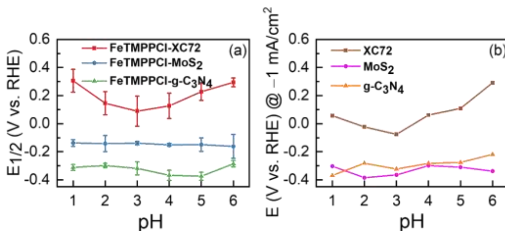
Figure 6. pH dependence of (a) E_{1/2} values from LSV of FeTMPPCl-XC72, FeTMPPCl-MoS 2 , and FeTMPPCl-g-C 3 N 4 and (b) ORR potential obtained at an ORR current density of -1 mA/cm 2 from LSV of bare XC72, MoS 2 , and g-C 3 N 4 .
