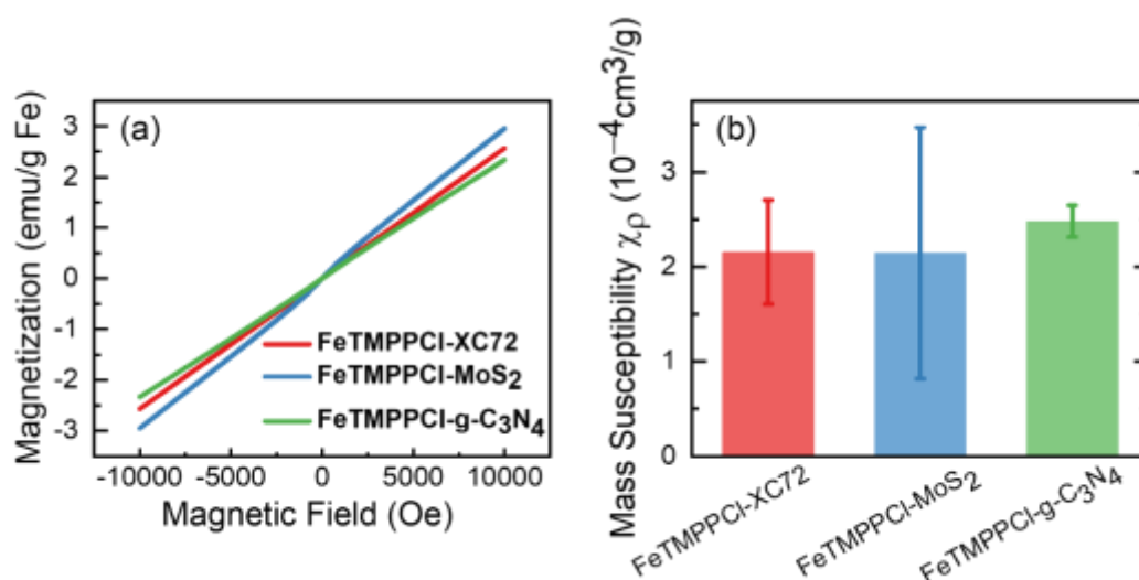
Figure 3. (a) SQUID Magnetometry and (b) susceptibility of FeTMPPCl-XC72, FeTMPPCl-MoS 2 , and FeTMPPCl-g-C 3 N 4 at 300 K (27 °C). Error bars represent standard deviation obtained from multiple measurements.
