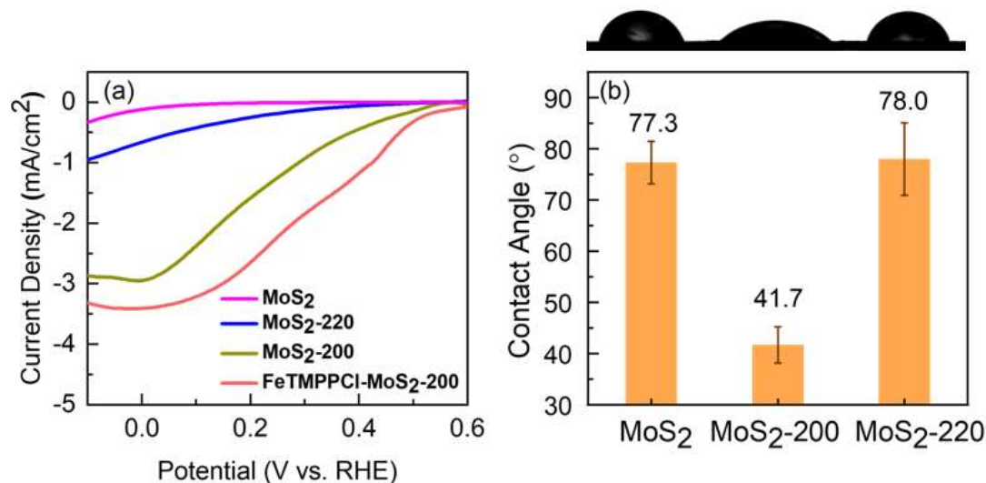
Figure 7. (a) Ar-subtracted LSV of MoS 2 , MoS 2 -220, MoS 2 -200, and FeTMPPCl-MoS 2 -200 obtained in 0.1 M HClO 4 at a rotation rate of 1600 rpm. (b) The average contact angle values for water measured on MoS 2 , MoS 2 -200 and MoS 2 -220 pellets.
