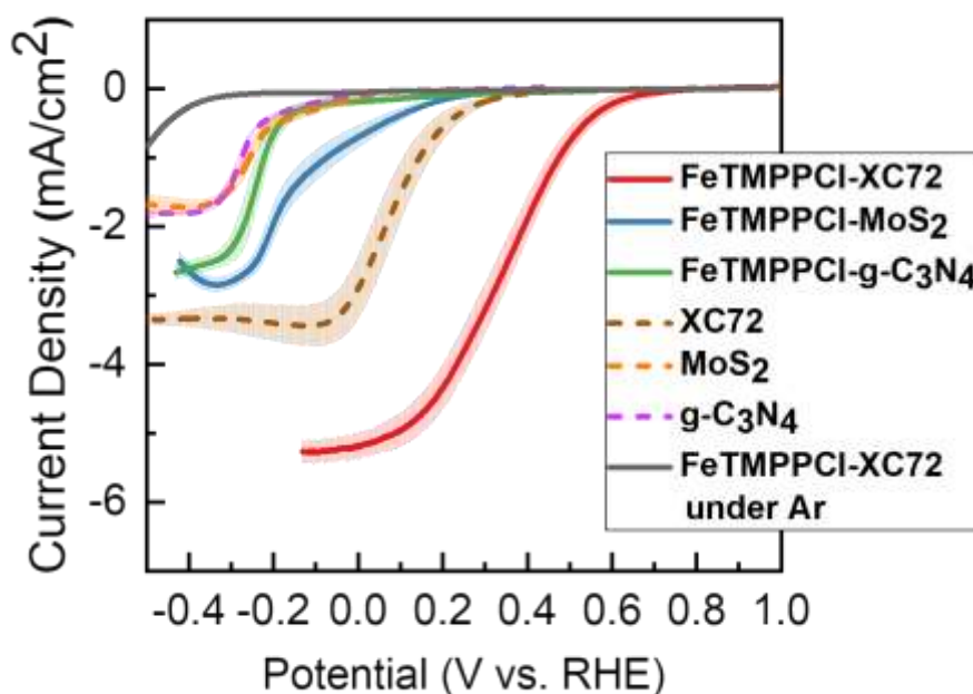
Figure 1. Ar-subtracted LSV obtained from FeTMPPCl-XC72, FeTMPPCl-MoS 2 , FeTMPPCl-g-C 3 N 4 , XC72, MoS 2 and g-C 3 N 4 in O 2 -saturated 0.1 M HClO 4 using an RDE at 1600 rpm. The shaded areas represent \pm one standard deviation in the current obtained from multiple measurements. The grey line was obtained from FeTMPPCl-XC72 in 0.1 M HClO 4 absent O 2 .
