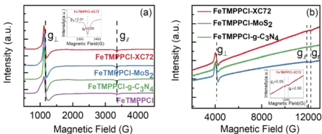
Figure 2. EPR of FeTMPPCl-XC72, FeTMPPCl-MoS 2 , and FeTMPPCl-g-C 3 N 4 obtained at 10 K: (a) X-band along with unsupported FeTMPPCl. The dashed lines demarcate g = 5.88 , 2.01 , and 2.00 (l-r). Inset: enlargement of 3220–3420 G field region of FeTMPPCl-XC72; (b) Q-band (solid state). The dashed lines demarcate g = 5.99 , 2.05 , and 2.00 (l-r). Inset: enlargement of 100350–13790 G field region of FeTMPPCl-XC72.
