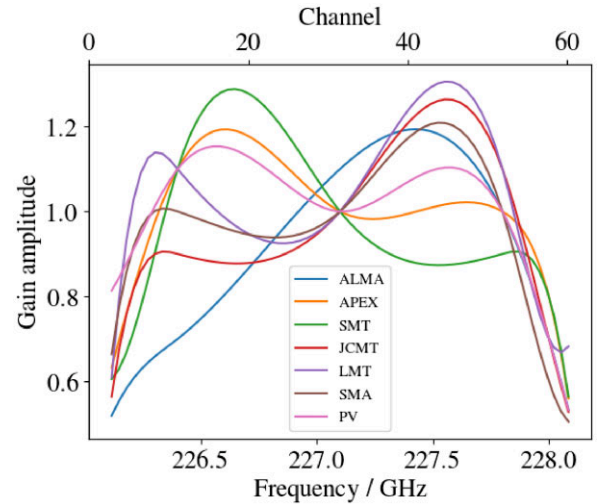
Figure 9. Station-based bandpass amplitudes used in generating synthetic data for Section 6.
