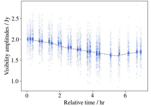
Figure 2. Stokes/visibility amplitudes for a point source with intrinsic time variability, as a function of time for one frequency channel.
