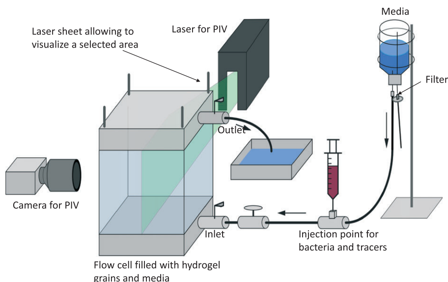
FIGURE 1 Experimental set-up. PIV = particle image velocimetry
