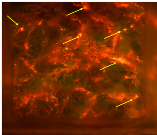
FIGURE 5 Bio-storage of solutes and particles into the extracellular polymeric substances (EPS) produced by the Sinorhizobium meliloti cells. Note the fluorescein and particles absorbed by the EPS structure after the drainage of the flow cell. This indicates the capability of microbe-produced substances to store solutes. Arrows point to areas where fluorescein was highly accumulated, which correspond to EPS and/or dead zones
