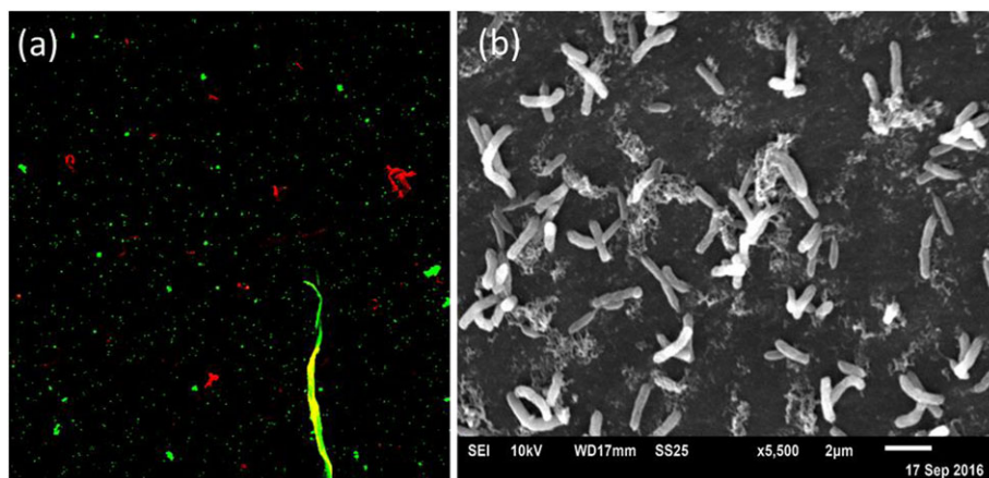
FIGURE 3 (a) Microbial (in green) and extracellular polymeric substance (in red) attachment on hydrogel surface using confocal imaging (field view 1.2 \times 1.2 mm) and (b) scanning electron microscopy
