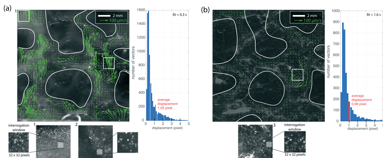
FIGURE 4 Flow-field measured (a) before biofilm formation and (b) after biofilm formation, when the flow cell was filled with hydrogel and media (M9). Inlets and histograms indicate the excellent quality of the particle image velocimetry for amended and unamended porous media
