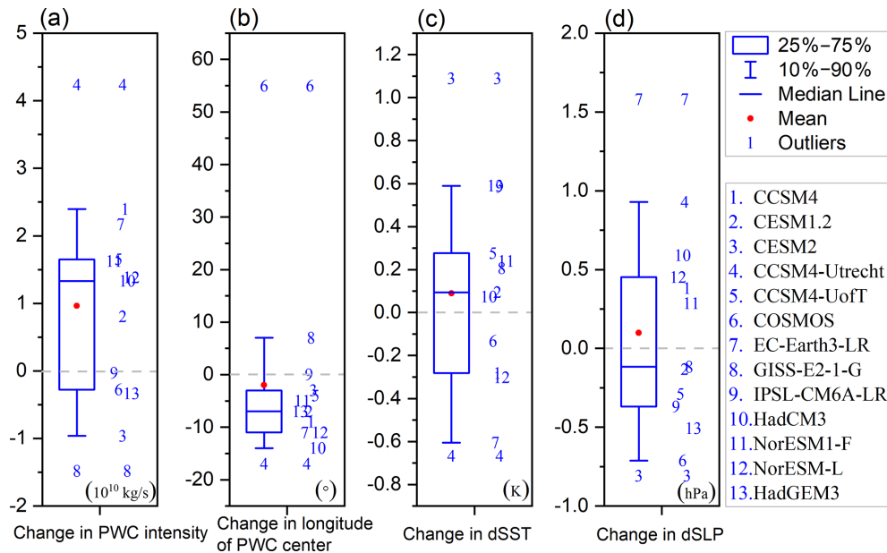
Figure 10. Changes in the annual mean of the (a) intensities of the Pacific Walker circulation (PWC; in 10^{10} \text{ kg s}^{-1} ), (b) longitude of the PWC cell center (in ^{\circ} ), (c) dSST (in K), and (d) dSLP (in hPa) for mid-Pliocene simulations compared with the PI simulation. Here, the PWC intensity is defined as the vertically integrated zonal mass stream function (ZMS; Bayr et al., 2014; Schwendike et al., 2014) averaged in the equatorial Pacific ( 140^{\circ} \text{ E} – 120^{\circ} \text{ W} ), and the location of the PWC cell center is the longitude of the maximum ZMS. The dSLP and dSST are defined as the difference in SLP and SST across the equatorial Indo-Pacific ( 160^{\circ} – 80^{\circ} \text{ W} , 5^{\circ} \text{ S} – 5^{\circ} \text{ N} minus 80^{\circ} – 160^{\circ} \text{ E} , 5^{\circ} \text{ S} – 5^{\circ} \text{ N} ).
