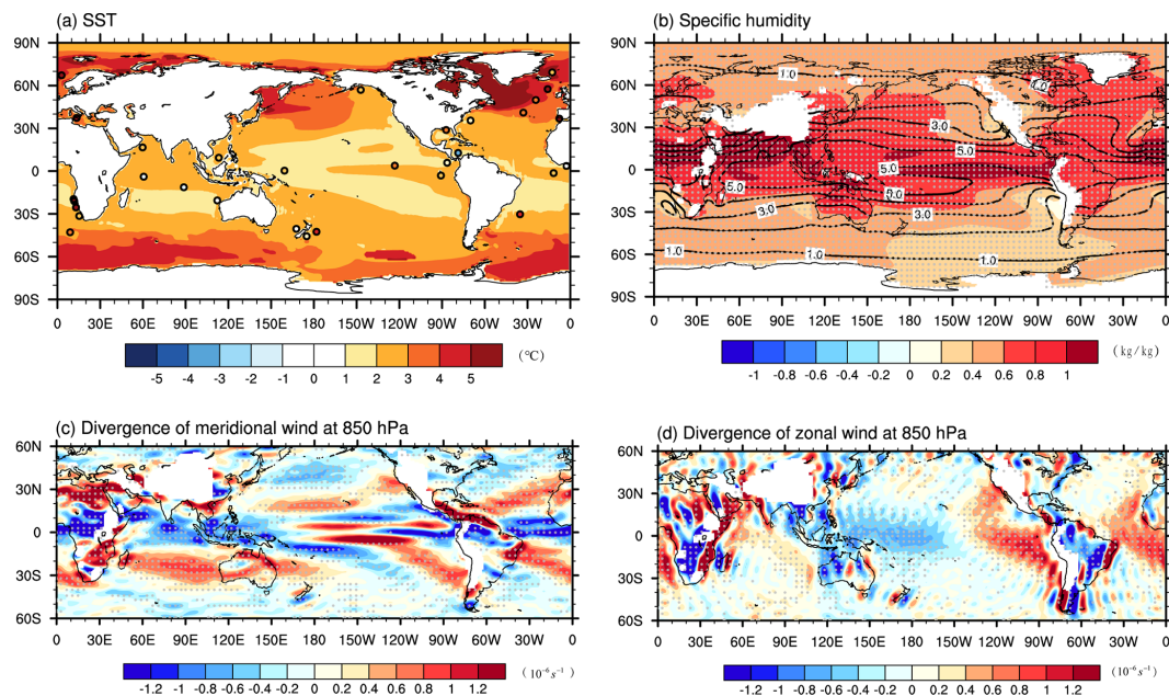
Figure 7. Change in (a) MMM SST (shading; in °C), and (b) specific humidity (shading; in \text{kg kg}^{-1} ) overlaid by its climate mean for the PI simulation. Panels (c) and (d) show the MMM divergence of the meridional V_M and zonal wind V_Z fields decomposed from the 3P-DGAC method at the 850 hPa level for the PI simulation (in 10^{-6} \text{ s}^{-1} ). The circles in panel (a) are the anomalies of reconstructed SST (McClymont et al., 2020) from the alkenone-derived U_{37}^{K'} index (Prahl and Wakeham, 1987) and foraminifera calcite Mg/Ca (Delaney et al., 1985). Stippling in panels (b–d) indicates regions where at least 10 of 13 simulations in the model group agree on the sign of the ensemble mean.
