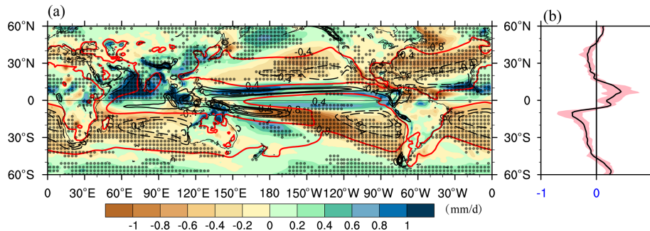
Figure 1. The simulated PmE changes in individual PlioMIP2 models. The zonal average of the PmE changes in each model is shown in panel (b) (units: \text{mm d}^{-1} ).
