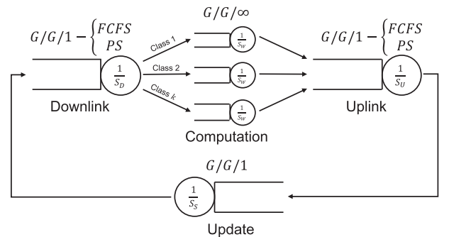
Fig. 5. Queueing Model of Async-SGD.
