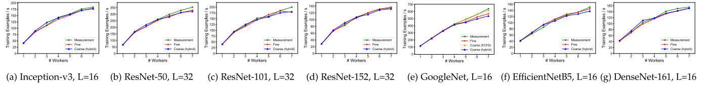
Fig. 16. Async-SGD without overlapping communication and computation on heterogeneous GPUs.
