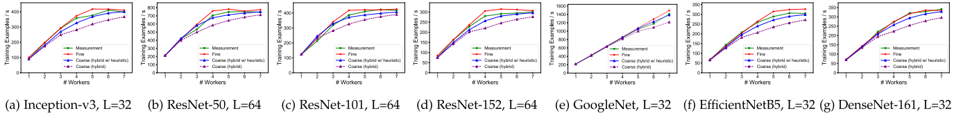
Fig. 15. Async-SGD with overlapping communication and computation on homogeneous GPUs.
