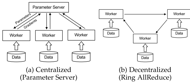
Fig. 1. Centralized and Decentralized Architectures.
