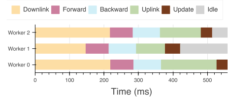
Fig. 7. Trace of Sync-SGD with 3 workers.
