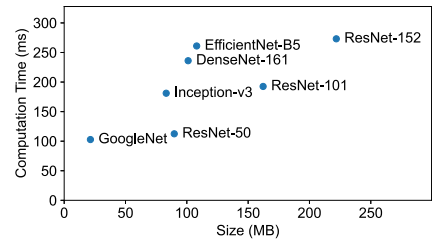
Fig. 11. Performance benchmark of neural network models with batch size 32 on Nvidia tesla V100 GPUs.
