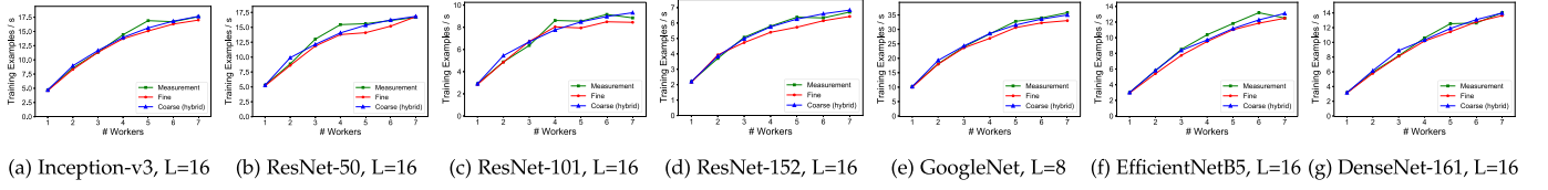
Fig. 12. Async-SGD without Overlapping Communication and Computation on Homogeneous CPUs.
