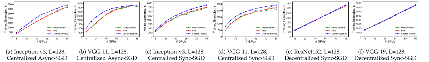
Fig. 22. Multi-GPU Experiments on AWS p3.16xlarge.
