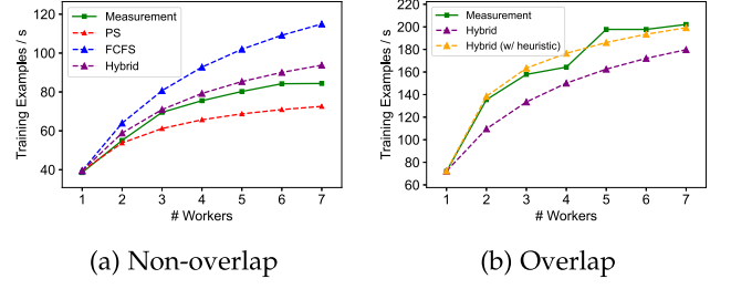
Fig. 9. Training ResNet-152 (batch size of 32 examples) on AWS p3.2xlarge with centralized Sync-SGD.
