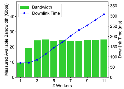
Fig. 23. Available bandwidth and downlink time on AWS 25Gbps network of the experiment in Fig. 22c.
