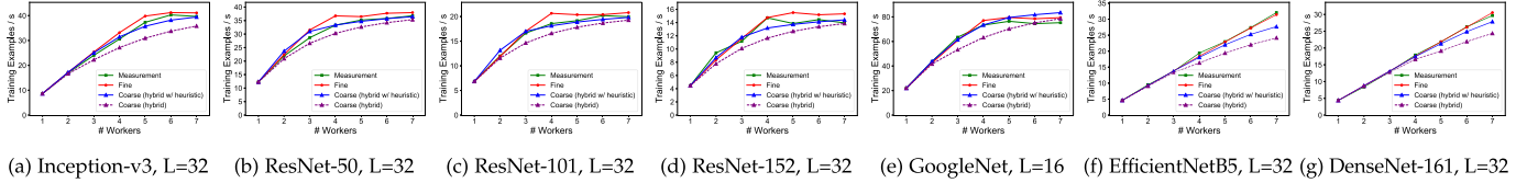
Fig. 14. Async-SGD with overlapping communication and computation on homogeneous CPUs.
