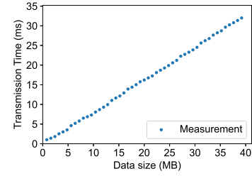
Fig. 6. Point-to-point transmission time for different data sizes on AWS 10Gbps network.
