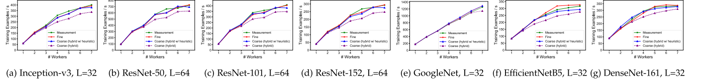
Fig. 17. Async-SGD with overlapping communication and computation on heterogeneous GPUs.
