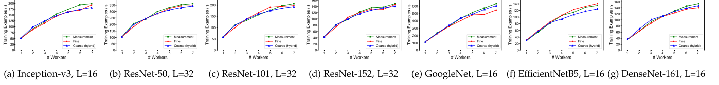
Fig. 13. Async-SGD without Overlapping communication and computation on homogeneous GPUs.
