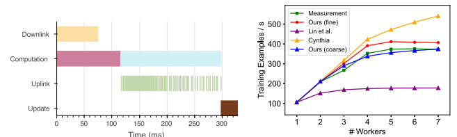
(a) Timeline of a Training Step (b) Comparison of Approaches
