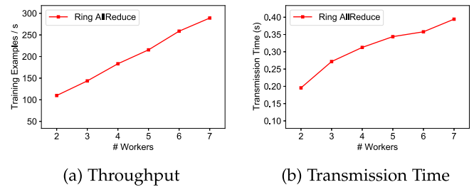
Fig. 3. Training ResNet-152 (batch size of 32 examples) on AWS p3.2xlarge with Ring AllReduce architecture.
