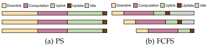
Fig. 8. Bandwidth sharing models in Sync-SGD.
