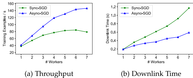
Fig. 2. Training ResNet-152 (batch size of 32 examples) on AWS p3.2xlarge with PS architecture.
