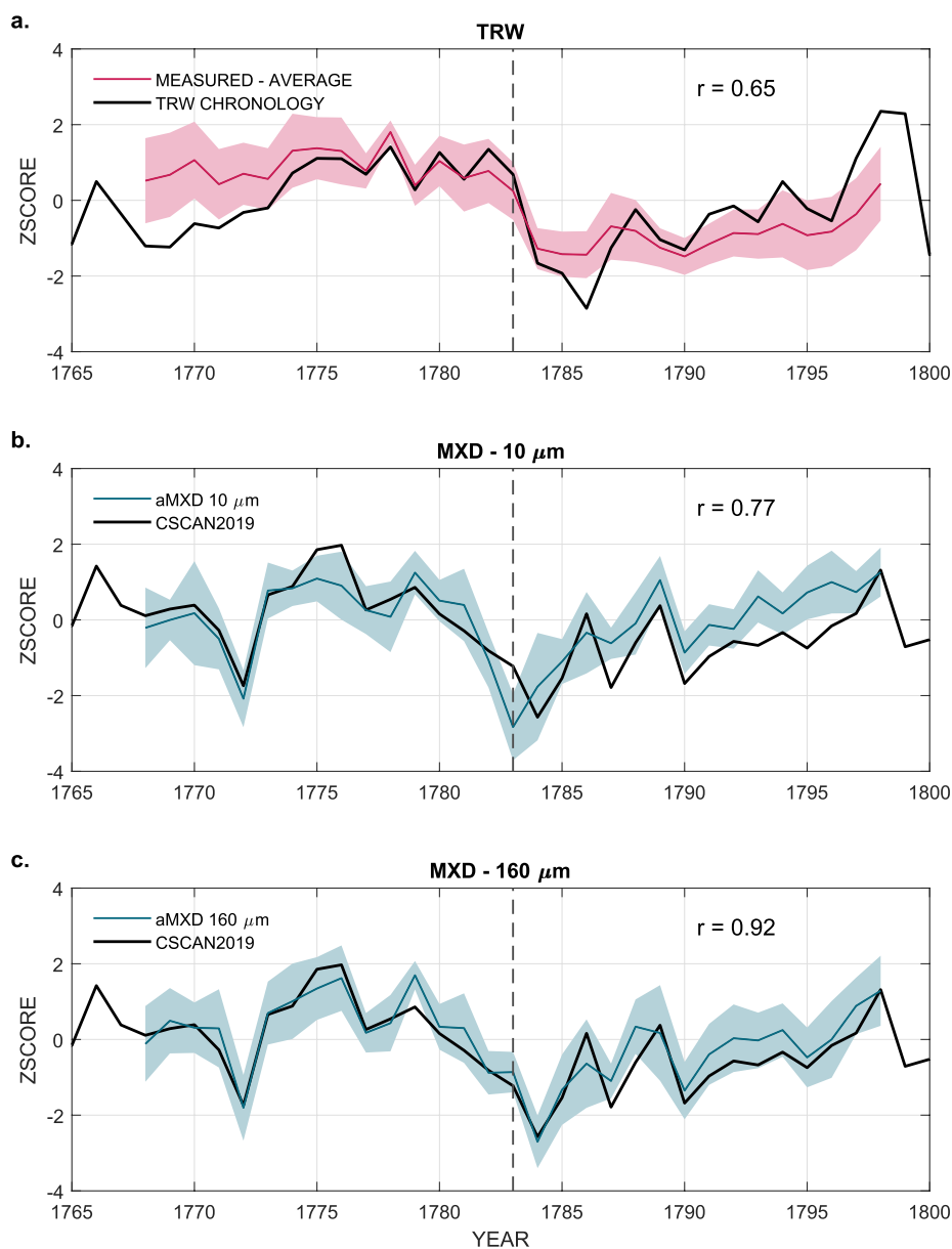
Figure 4. (a) Full sample ( N = 24 ) tree-ring width (TRW) chronology (black line) and average tree-ring width of samples measured in ROXAS ( N = 9 , red line). (b), (c) Updated CSCAN2019 MXD chronology (black line) from Linderholm and Gunnarson (2019) and the anatomical MXD (aMXD) measurements (blue line) at a resolution of 10 \mu (b) and 160 \mu (c). Results from the Pearson correlation coefficient calculations are included in each plot. Values are normalized for comparison of the related, but different, measurements. The data in this study were analyzed over the 30-year period: 1768–1798. Shaded regions show the \pm 1 SD around the mean values. None of the anatomical chronologies were detrended. The aMXD10 has a lower correlation with the CSCAN2019 MXD chronology because of the drop in density in the last part of the ring that is captured by the high-resolution aMXD.
