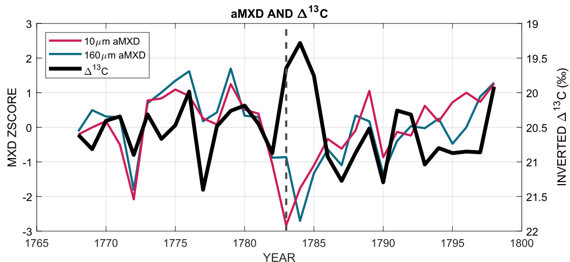
Figure 10. Times series of \Delta^{13}\text{C} (black) converted from (Seftigen et al., 2011) and aMXD chronologies at the 10 \mu\text{m} resolution (red) and at the 160 \mu\text{m} resolution (blue). aMXD chronologies are normalized. The \Delta^{13}\text{C} time series axis is inverted for better visual interpretation.
