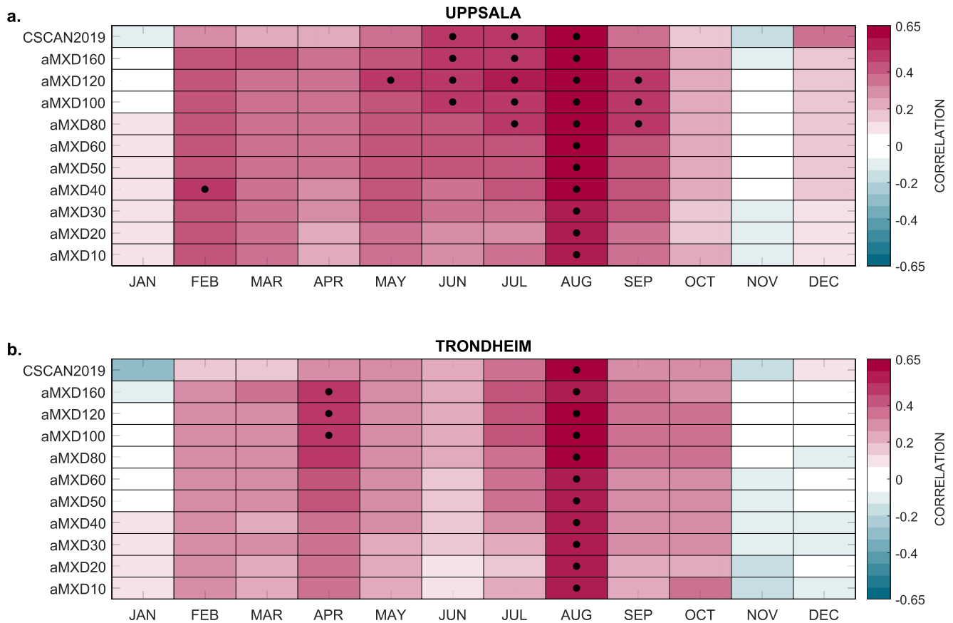
Figure 9. Results from the Pearson correlation coefficient calculations between the monthly data at Uppsala (a) and Trondheim (b), and the multiple resolution aMXD and CSCAN2019 MXD chronologies from 1768 to 1798 CE. Significant correlations ( \alpha = 0.01 ) are indicated with a dot.
