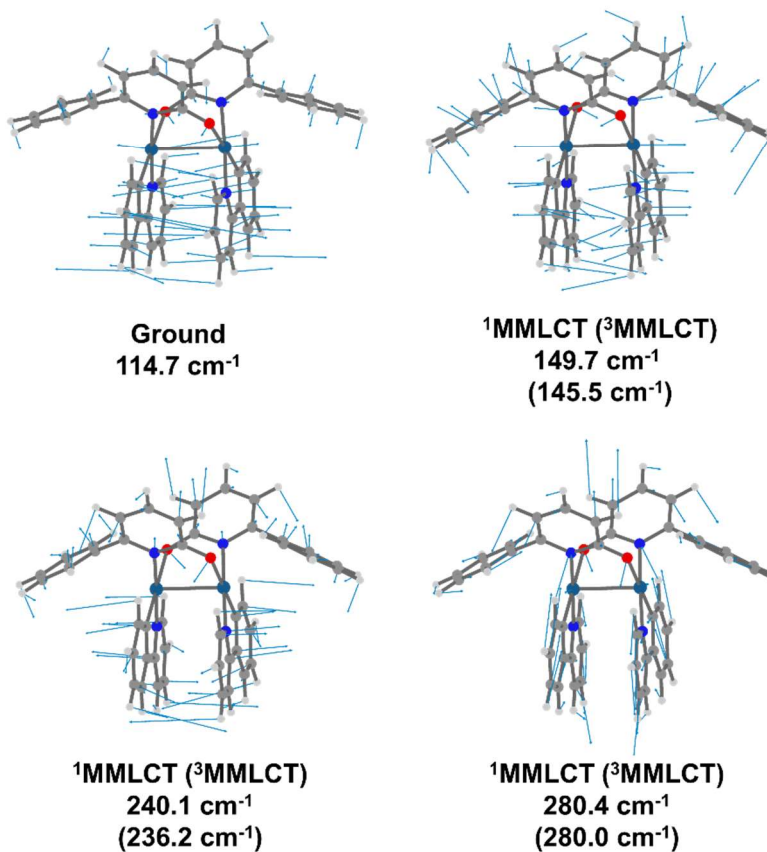
Figure 4. (a) Optimized molecular structures for ground-, 1 MMLCT and 3 MMLCT states. The red dotted arrows highlight the decrease in the twisting angle between the ppy ligand planes. (b) calculated normal modes for ground-, 1 MMLCT and 3 MMLCT states.
