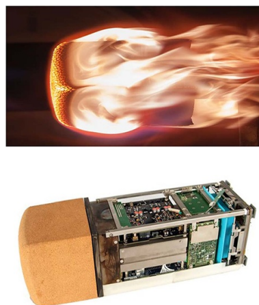
Figure 26. Top: ablative material testing in the plasmatron facility of the von Karman Institute For Fluid Dynamics ( 16 \text{ g s}^{-1} air mass flow, 10 000 Pa pressure, 2.5 \text{ MW m}^{-2} calorimeter heat flux) for the QARMAN ablative heatshield made of cork P50 from Amorim TM . Bottom: QARMAN ( 34 \times 10 \times 10 \text{ cm}^3 ) platform with INES payload including emission spectrometer and photodiode to measure simultaneously the shock layer radiation and ablative material recession.
