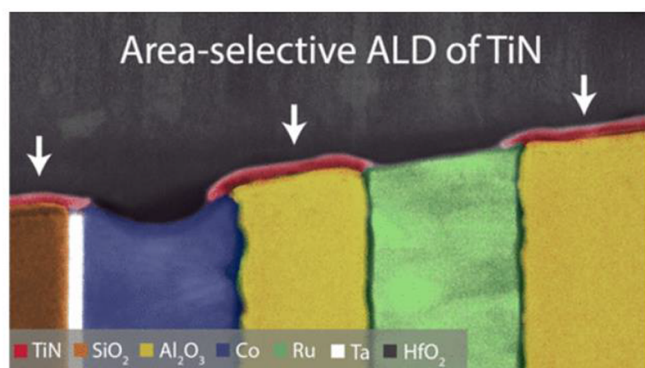
Figure 9. Demonstration of selective deposition ~6 nm TiN on SiO 2 and Al 2 O 3 areas of a nanoscale pattern with Co and Ru non-growth areas. Reproduced with permission from [69]. CC BY-NC 4.0.
