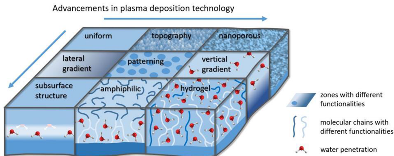
Figure 14. Representation of advanced surface functionalities important for biomaterials. While surface modifications are well studied, the controlled structuring of the near-surface region enables novel surface characteristics based on the combination of different functionalities and related water interaction.
