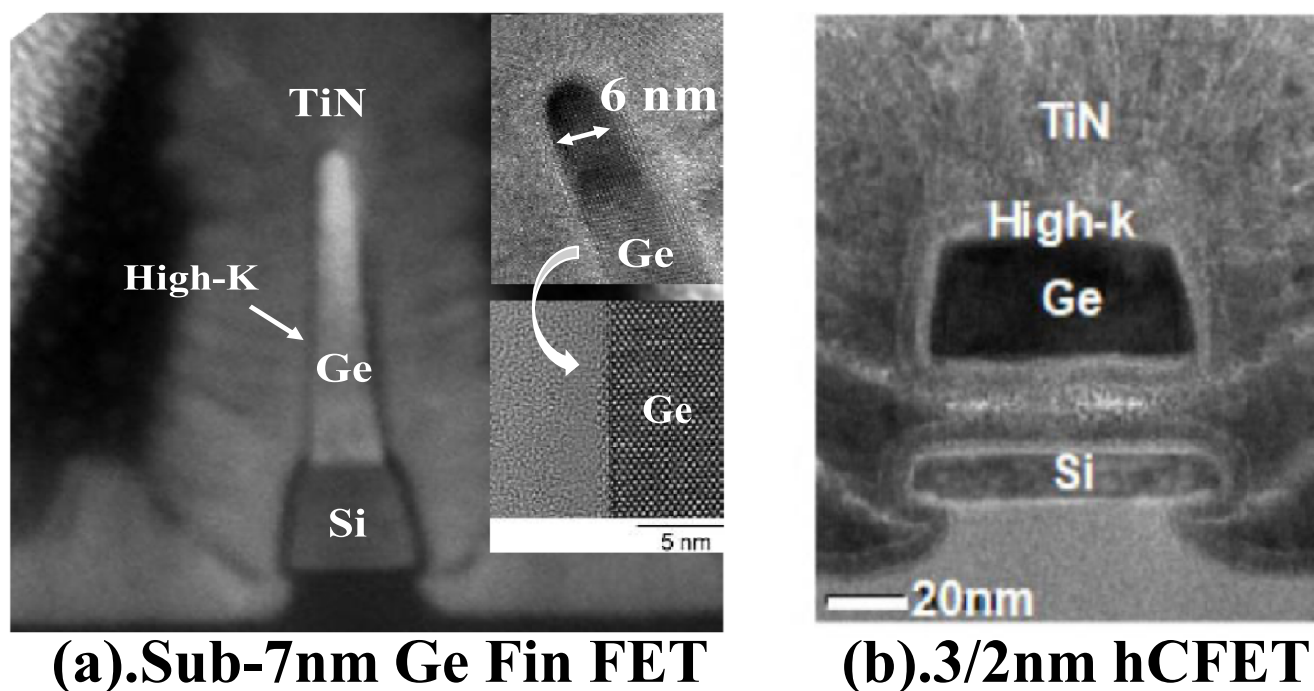
Figure 8. Advanced complementary metal-oxide-semiconductor (CMOS) devices fabricated by NDALE. © 2007 IEEE. Reprinted, with permission, from [65]. © 2004 IEEE. Reprinted, with permission, from [66].
