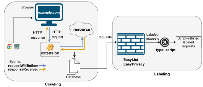
Figure 2: TRACKERSIFT's web crawling and labeling
