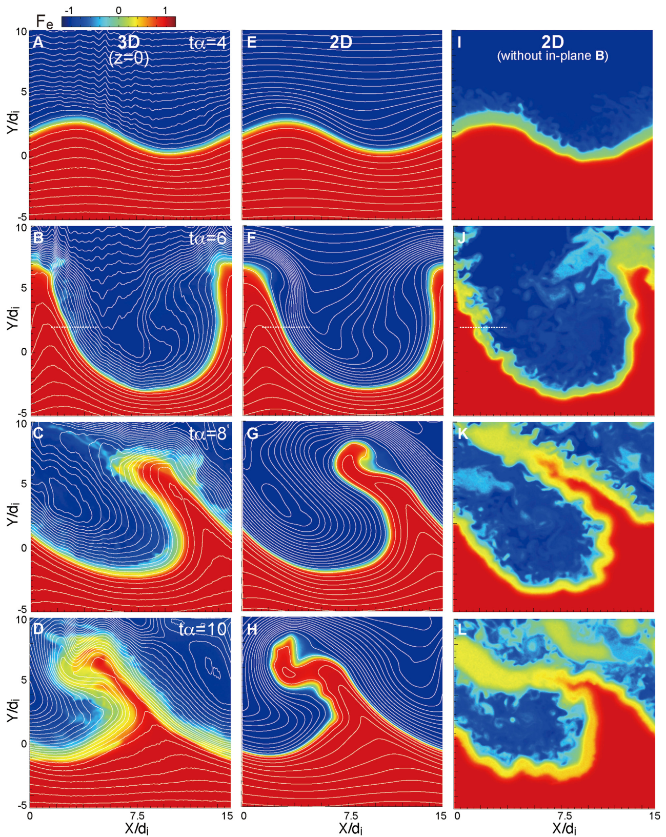
FIGURE 1 | Time evolution of the mixing measure F_e = (n_{e1} - n_{e2}) / (n_{e1} + n_{e2}) in the x - y plane ( z = 0 for the 3-D run) for the 3-D ( A–D ), the corresponding 2-D ( E–H ), and 2-D without initial in-plane fields ( I–L ) runs. The white curves for the 3-D and corresponding 2-D runs show the surfaces of the z -component of the vector potential, which corresponds to the in-plane magnetic field lines in 2-D.
