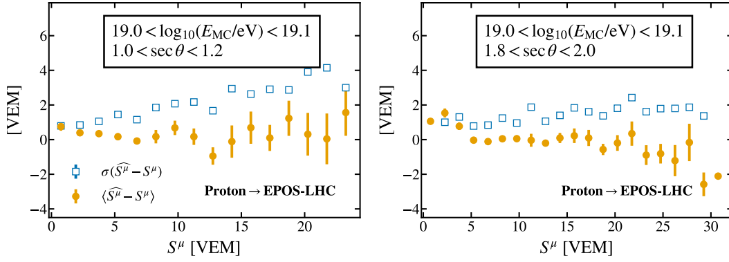
Figure 10. Mean and standard deviation of the difference between the integral of the predicted muon signal \widehat{S}^\mu and the integral of the true muon signal S^\mu for all the stations from events with the energies and zenith angles specified in the boxes.
