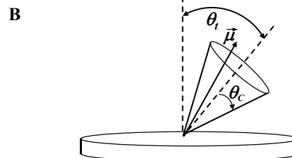
Figure 6. (A) Anisotropy decay of the \text{S}^{12}\text{CN}^- anions of \text{Cs}_2\text{Pb}(\text{S}^{12}\text{CN})_2\text{Br}_2 . The decay for the \text{I}^- perovskite is similar. The data are horizontal within experimental error, demonstrating that after ultrafast librational motions, there is no further orientational relaxation. (B) Schematic of the wobbling-in-a-tilted-cone model. The cone axis is tilted by \theta_t from the planar surface normal. The wobbling (librational) cone half angle is \theta_c .
