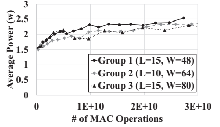
Fig. 7: Average power consumption for different CONV models
