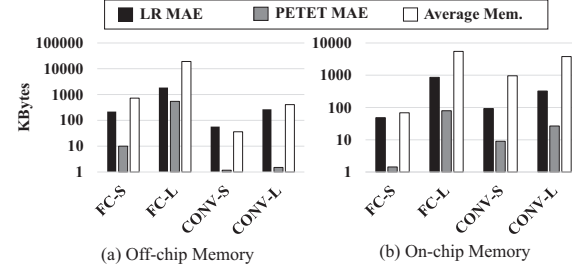
Fig. 10: Summary of memory usage estimation errors
