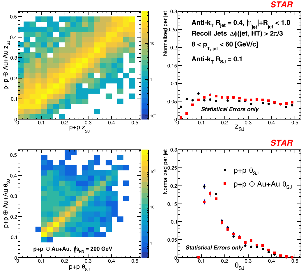
FIG. 7. Left panels: Correlation studies of the two subjet observables z_{SJ} (top row) and \theta_{SJ} (bottom row) similarly to Fig. 4. Right panels: The projections along x and y axes shown with only statistical errors.
