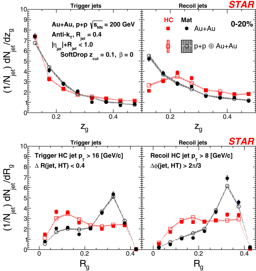
FIG. 3. Distributions of softDrop z_g (top) and R_g (bottom) for trigger (left) and recoil (right) jets for Au + Au data (filled symbols) and the p + p \oplus \text{Au} + \text{Au} reference (open symbols). The shaded regions represent systematic uncertainty in the embedded reference. The red and black points represent HardCore and Matched jets, respectively.
