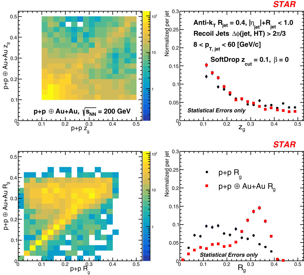
FIG. 4. Left panels: Correlation studies due to the heavy-ion underlying event for SoftDrop z_g (top) and R_g (bottom). Right panels: The projections along the x and y axes shown with only statistical errors.
