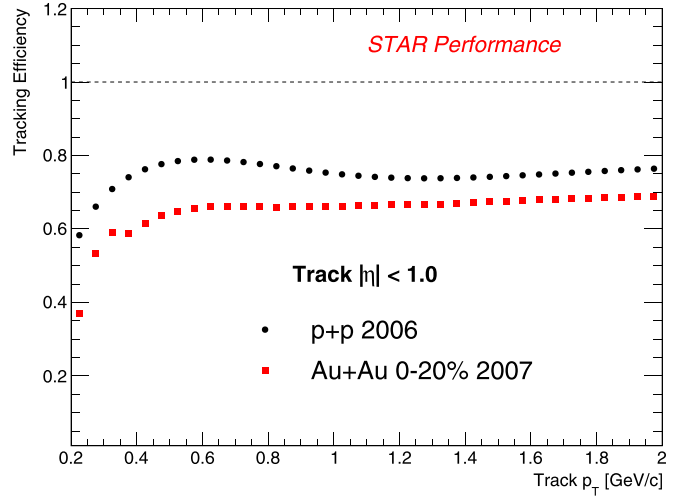
FIG. 11. TPC tracking efficiencies for the 2006 p + p and 2007 Au + Au datasets utilized in the embedding studies for tracks within |\eta| < 1.0 .
