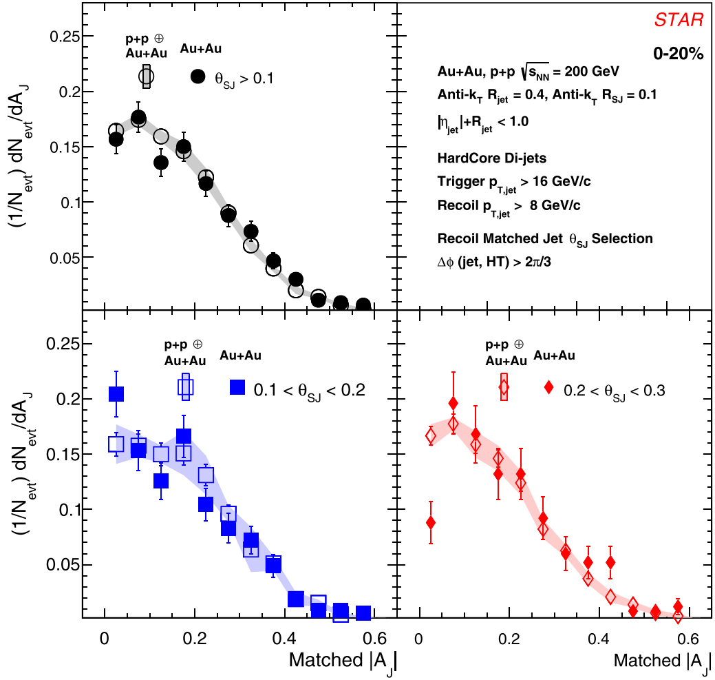
FIG. 10. Distributions of Matched dijet asymmetry ( |A_J| ) for events with leading and subleading cuts of 16 and 8 GeV/c (for HardCore jets), respectively. The filled markers correspond to Au + Au data and the open markers along with the shaded regions show p + p \oplus Au + Au reference. The black distributions do not have any cuts on the subjet \theta_{SJ} , whereas for the blue and red distributions, selections on recoil Matched jets with 0.1 < \theta_{SJ} < 0.2 and 0.2 < \theta_{SJ} < 0.3 are applied. The vertical error bars represent statistical uncertainty on the data points.
