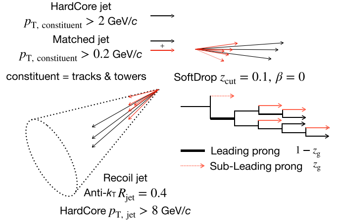
FIG. 2. Visualization of the SoftDrop declustering step applied on a recoil jet resulting in the selection of the leading and subleading prongs.
