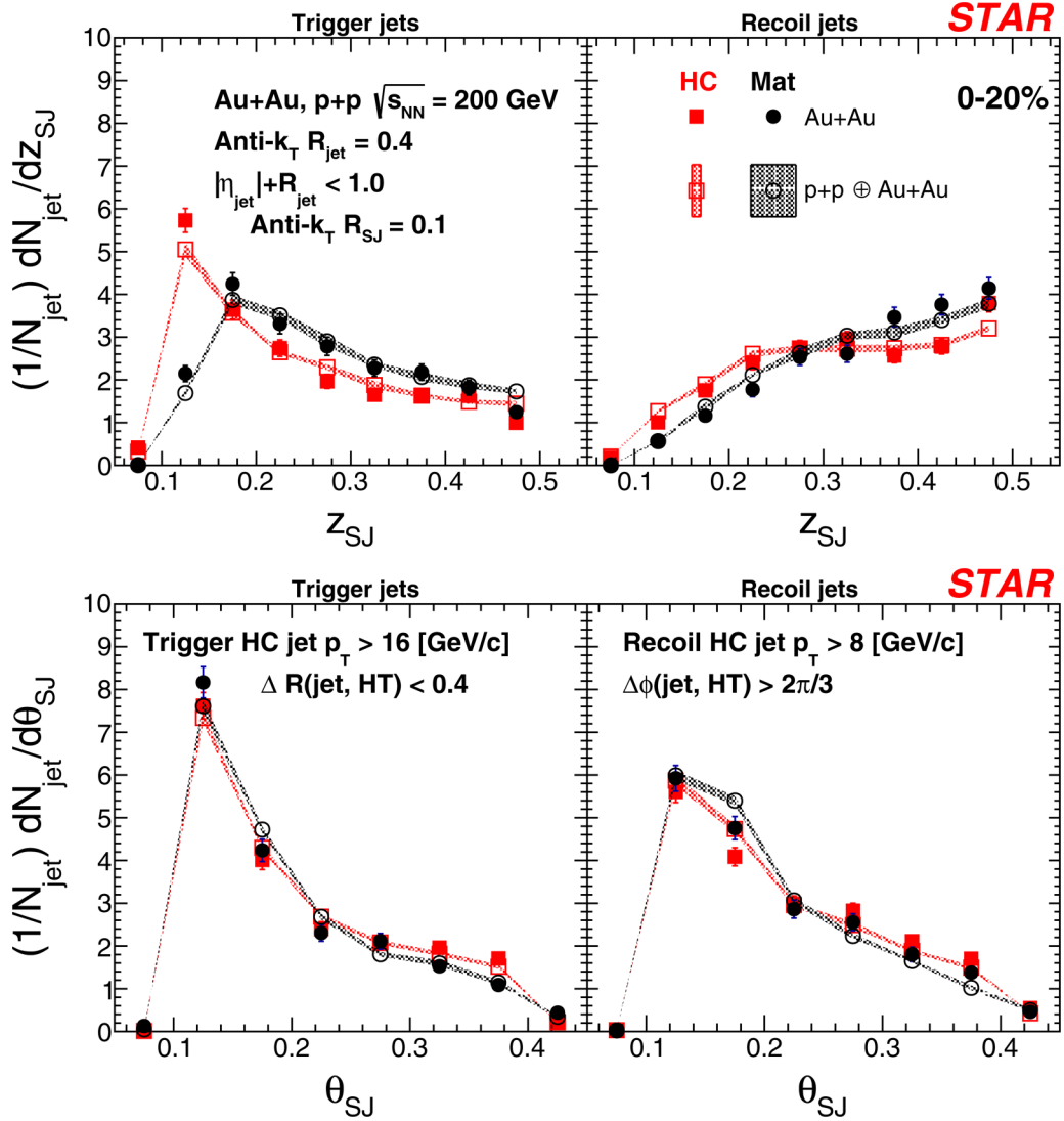
FIG. 8. Distributions of subjet observables z_{SJ} (top) and \theta_{SJ} (bottom) for trigger (left panels) and recoil (right panels) jets. The Au + Au plots are shown in the filled markers whereas the open markers represent p + p \oplus \text{Au} + \text{Au} which includes the shaded regions representing systematic uncertainty. The red and black points represent HardCore and Matched jets, respectively.
