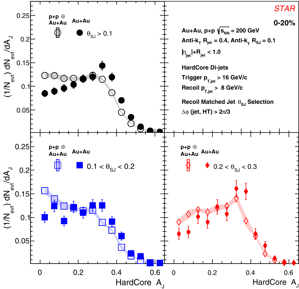
FIG. 9. Distributions of HardCore dijet asymmetry ( A_J ) for events with leading and subleading cuts of 16 and 8 GeV/c, respectively. The filled markers correspond to Au + Au data and the open markers along with the shaded regions show p + p Au + Au reference. The black distributions do not have any cuts on \theta_{SJ} , whereas for the blue and red distributions, selections on recoil Matched jets with 0.1 < \theta_{SJ} < 0.2 and 0.2 < \theta_{SJ} < 0.3 are applied. The vertical error bars represent statistical uncertainty on the data points.
