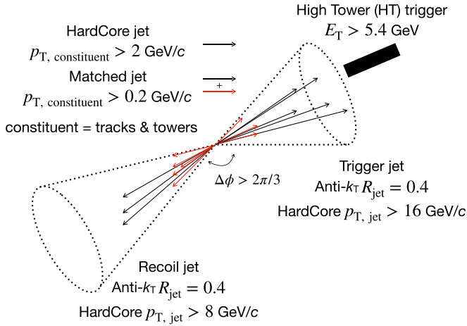
FIG. 1. Description of the dijet event selection noting the trigger and recoil jets along with the HardCore and Matched jets which include the hard and soft constituents in the black and red colored arrows, respectively. The high tower trigger is shown in the thick black shaded region in the trigger jet region. The thrust axes for HardCore and Matched jets can be slightly different since they are associated via \Delta R matching criterion.
