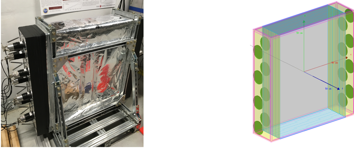
Figure 1. Left: a photograph of the MARS detector in Neutrino Alley. The bases of the PMTs are visible on the left-hand side of the photograph, and a unistrut support structure holds the stacked scintillators. Right: Geant4 [11] model of the detector. The cyan boxes represent the plastic scintillator layers. The side acrylic light guides are in yellow, with green circles representing the PMT windows.
