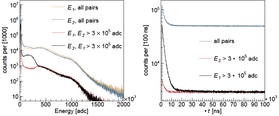
Figure 5. Left: histograms of the first pulse’s energy E_1 and the second pulse’s energy E_2 of the scintillator pulse pairs from the April 2018 beam-off data. The first two histograms in the legend include all pairs. The last (black) E_2 histogram only includes pairs with E_1 > 3 \times 10^5 adc that select muon-track high-energy depositions. The (red) E_1 histogram, with the same cut applied instead to E_2 , illustrates the differences in the E_1 and E_2 populations. Right: histograms of the inter-pulse time \Delta t for the same cuts. The black histograms of both panels clearly show the spectral ( E_2 ) and time ( \Delta t ) profiles expected for Michel electrons.
