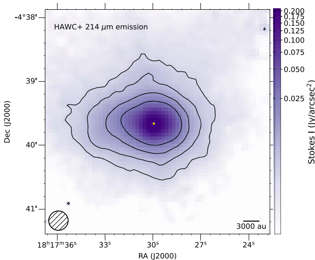
Figure 8. Total intensity of 214\ \mu\text{m} emission of L483. Contours at 3\sigma , 5\sigma , 10\sigma , and 20\sigma , where \sigma = 1.4\ \text{mJy arcsec}^{-2} . The Band E beam ( 18.2\ \text{arcsec} ) is shown in the bottom left. The position of the ALMA protostar is shown as a yellow star.
