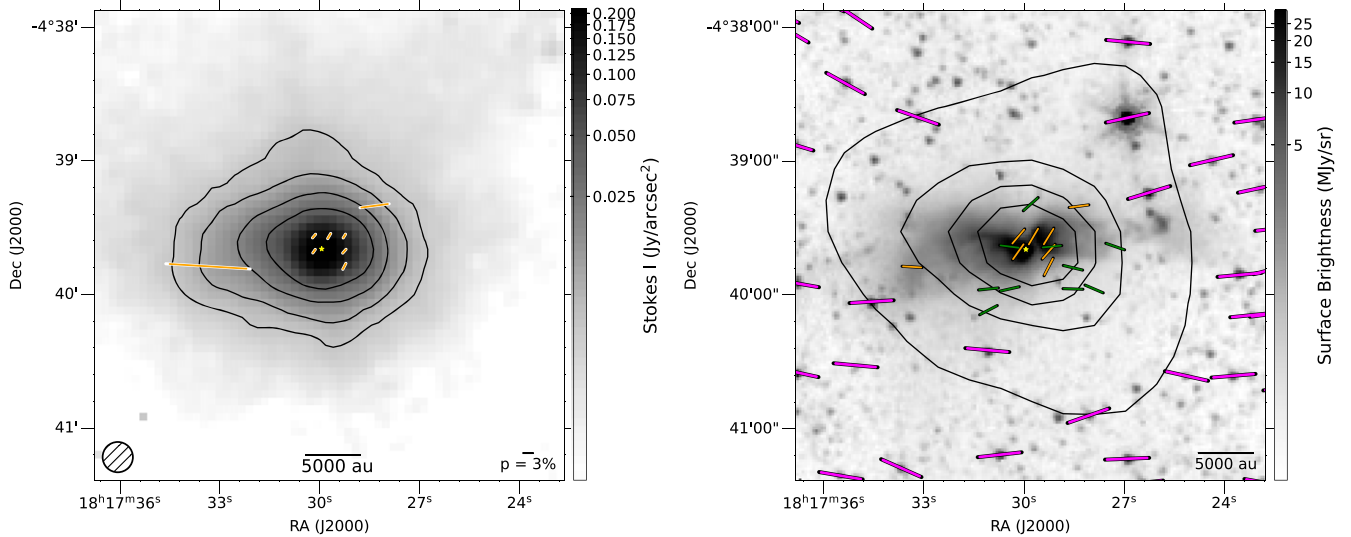
Figure 2. Left: SOFIA Band D (154 \mu\text{m} ) observations of L483. The 154 \mu\text{m} total intensity emission is shown in gray scale and contours. The black contours are shown at 3\sigma , 5\sigma , 10\sigma , and 20\sigma , where \sigma = 1.9 \text{ mJy arcsec}^{-2} . Scaled magnetic field vectors in orange with the polarization percentage scale bar shown on the bottom right. The inner vectors have a polarization \geq 1\% , while the two outer vectors are 7% and 20.4%. The resolution of the observations is \sim 13''.6 and is shown on the bottom left. Right: a subset of the H -band vectors (magenta) shown on the Spitzer 4.5 \mu\text{m} background image. SHARP 350 \mu\text{m} (Chapman et al. 2013) vectors are shown in green and HAWC+ 154 \mu\text{m} vectors are shown in orange. Note that the HAWC+ vectors are Nyquist sampled, while the SHARP vectors correspond to independent beams. All vectors shown are inferred magnetic field orientation. Both panels show the location of the ALMA protostar as a yellow star.
