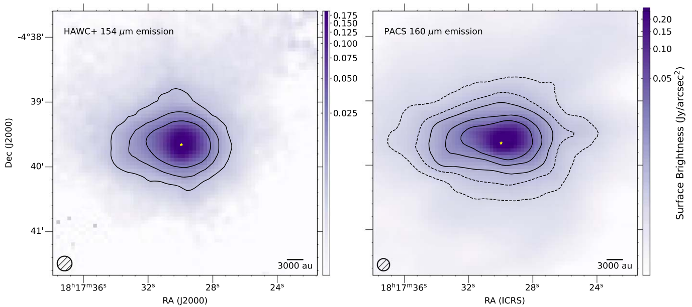
Figure 3. Left: HAWC+ 154 \mu\text{m} total intensity shown in the color scale and contours. The solid black contours shown correspond to 6, 12, and 25 \text{mJy arcsec}^{-2} . The \sim 13'' beam is shown in the bottom left. Right: PACS 160 \mu\text{m} L483 data shown in the color scale and contours. The PACS \sim 11'' beam is shown in the bottom left. We show dashed black contours corresponding to 2.5 and 4 \text{mJy arcsec}^{-2} , and solid black contours at 6, 12, and 25 \text{mJy arcsec}^{-2} . To compare the source shape between the two telescopes we plot the same contours on the HAWC+ data (6, 12, and 25 \text{mJy arcsec}^{-2} ), excluding the two levels that are lower than the sensitivity of the HAWC+ data. The shape of L483 is elongated in the N–S direction in the 154 \mu\text{m} data compared to the 160 \mu\text{m} data. This is expected due to the nature of chop–nod observations. In both images we show the location of the ALMA protostar with a yellow star.
