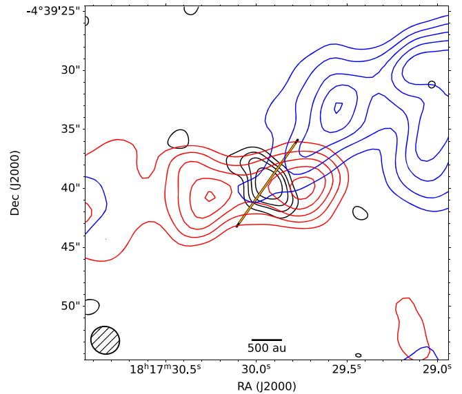
Figure 5. Flattened infall envelope of L483 shown in black contours from 870\ \mu\text{m} SMA observations (Leung et al. 2016). The beam of the SMA data ( \sim 2'' \times 35'' ) is shown in the bottom left corner. Contours are shown at 3\sigma , 5\sigma , 7\sigma , and 10\sigma , where \sigma is 3.4\ \text{mJy beam}^{-1} . The outflow at 4'' resolution in ^{12}\text{CO} (1–0) from OVRO is seen in the red and blue contours (Velusamy et al. 2014). The red and blue contours are spaced 0.4\ \text{Jy beam}^{-1} . The unweighted mean of six measurements of field direction at 154\ \mu\text{m} is shown in the orange vector.
