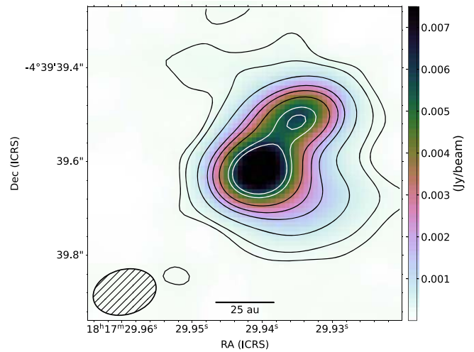
Figure 9. ALMA image of L483 using robust = 0.5 weighting. Black contours at 6\sigma , 10\sigma , 25\sigma , 50\sigma , 70\sigma , and 100\sigma , where \sigma = 33\ \mu\text{Jy beam}^{-1} . White contours show 150\sigma and 175\sigma .
