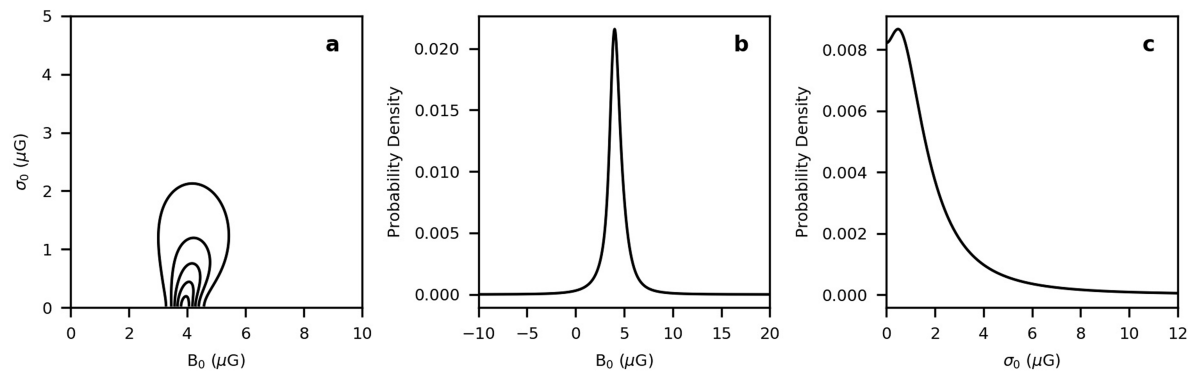
Extended Data Fig. 1 | Likelihood \mathcal{L} for the coherent magnetic field to have mean ( B_0 ) and spread ( \sigma_0 ) values. a, Contours of \mathcal{L} as functions of B_0 and \sigma_0 plotted at 10%, 30%, 50%, 70% and 90% of the peak value. b, The probability
