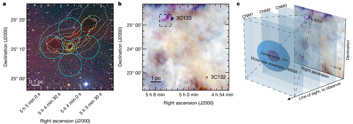
Fig. 1 | L1544 core and illustration of the structure of interstellar medium from the CNM to the core. a , A composite of Digitized Sky Survey 2 (DSS2) images of L1544 with the i band in red, the r band in green and the b band in blue overlaid with the HINSA and H 2 column density maps. The white dashed contours are 30%, 50%, 70% and 90% of the peak HINSA column density, and the orange contours are 2 \times 10^{21} \text{ cm}^{-2} , 4 \times 10^{21} \text{ cm}^{-2} , 6 \times 10^{21} \text{ cm}^{-2} , 8 \times 10^{21} \text{ cm}^{-2} and 10 \times 10^{21} \text{ cm}^{-2} for the H 2 column density. The red, green and cyan circles mark
