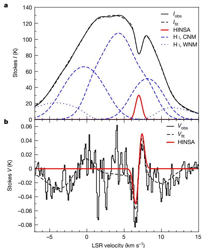
Fig. 2 | The Stokes I(\nu) and V(\nu) spectra at 21-cm wavelength towards the HINSA column density peak. a , The black profile represents the I(\nu) spectrum. The red profile represents the absorption from the foreground HINSA component. The blue dashed and dotted profiles represent the emission from the CNM and WNM components, respectively. The CNM and WNM profiles include the absorption from the CNM components that lie in front but do not include the absorption from the HINSA. The black dashed profile represents the sum of the absorption and emission profiles. b , The black profile represents the V(\nu) spectrum. The black dashed profile represents the sum of the Zeeman splitting profiles of the five components. The red profile represents the Zeeman splitting profile with B_{\text{los}} = +3.8 \mu\text{G} of the HINSA component.
