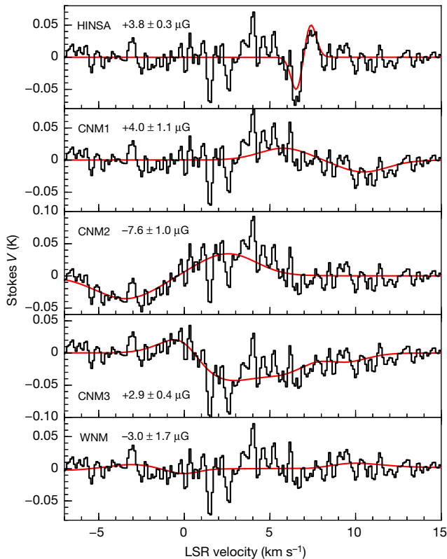
Fig. 3 | The individual V(v) profiles for the HINSA, CNM and WNM components. In each panel, the red profile represents the fitted Zeeman profile of the component and the black profile represents the observed V(v) subtracted by the fitted Zeeman profiles of the other four components. The CNM and WNM Zeeman profiles include the absorption from the CNM components that lie in front but do not include the absorption from the HINSA. The sum of the red profiles of the five components is the black dashed profile in Fig. 2b.
