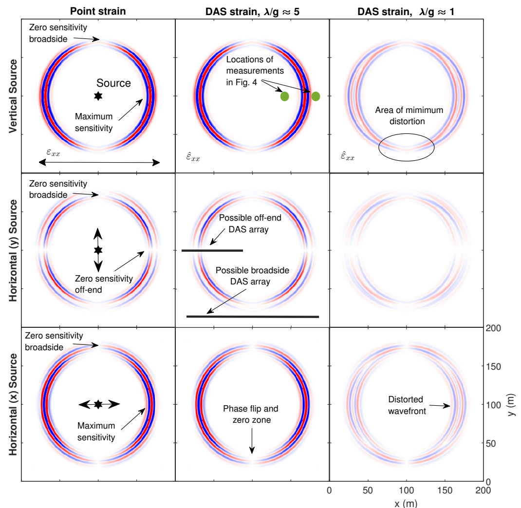
Figure 3. Simulations of normalized pointwise ( \epsilon_{xx} ) and distributed ( \hat{\epsilon}_{xx} ) strain in the x-direction at the top surface of a 200 m by 200 m by 100 m elastic half-space model caused by a 100 kN force. The strain is shown as measured by an ideal distributed strain sensing system aligned in the x-direction with wavelength-to-gauge length ratios ( \lambda/g ) of 5 and 1. This is approximately what DAS would measure neglecting effects from the pulse shape and cable transfer functions. Each source with horizontal polarization began their Ricker wavelet source signal in the positive x or y-direction. The source is shown centered in the model to demonstrate the theoretical pointwise strain and corresponding distributed measurements at all angles. All tiles are normalized relative to the maximum strain across all simulations. The simulations were conducted using Seismic Waves 4th Order [39].
