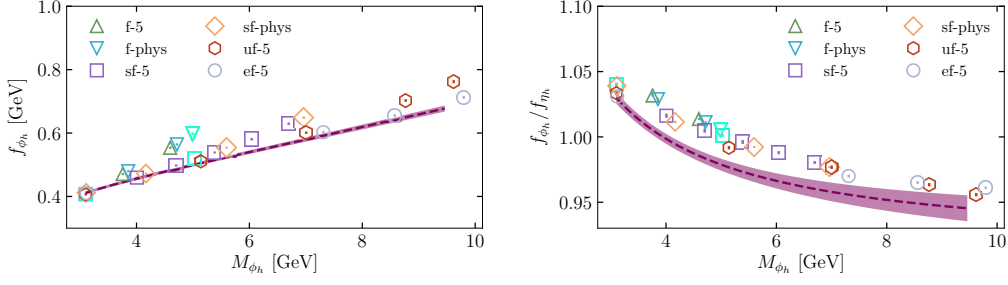
Figure 2: The left-hand plot shows the decay constant of the vector heavyonium meson as a function of its mass from n_f = 2 = 1 + 1 lattice QCD [1]. The points are the lattice results (with symbols as in Figure 1) and the purple band shows a model-independent fit using cubic splines. The right-hand plot shows the ratio of vector to pseudoscalar decay constants as a function of the vector heavyonium mass. Some systematic errors, such as discretisation effects, largely cancel in this ratio. This makes it very clear that the ratio changes from being greater than 1 to being less than 1 as the heavy quark mass is increased from c to b .
