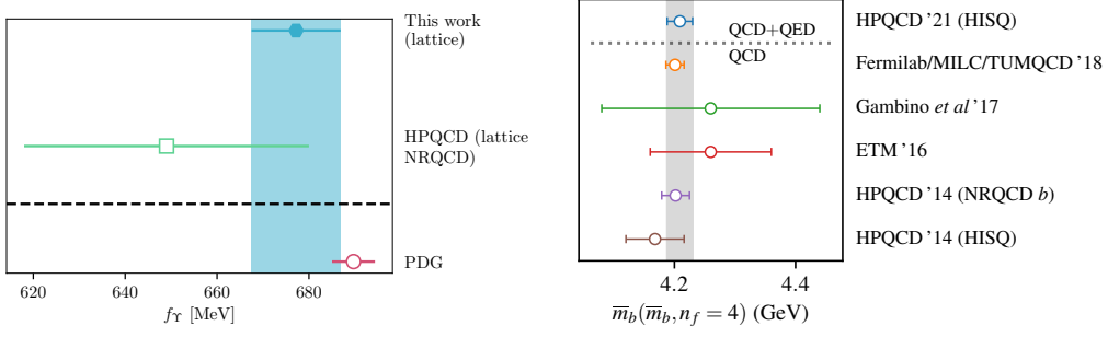
Figure 4: The left-hand plot compares our result (filled blue hexagon) for the \Upsilon decay constant to an earlier HPQCD result using NRQCD b quarks [13] (green open square). Our result, carried down as the blue band, is also compared to the experimental average result [8], inferred from the \Upsilon leptonic width, given by the pink open circle. We see good agreement with experiment at the level of our 1.4% uncertainty. The right-hand plot compares our new value for m_b in QCD+QED to earlier results that used lattice QCD calculations, estimating QED effects. These earlier results are from [13–17].
