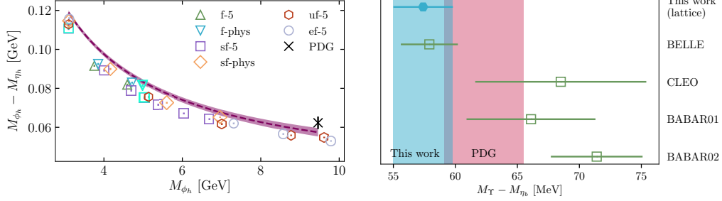
Figure 1: The left-hand plot shows the heavyonium hyperfine splitting as a function of the vector heavyonium mass from n_f = 2 + 1 + 1 lattice QCD [1]. The range covered is from the c quark mass to the b quark mass. Points show lattice QCD results at a range of lattice spacings from 0.09 fm (denoted f), through 0.06 fm (denoted sf) and 0.045 fm (denoted uf) to 0.03 fm (denoted ef). Sea u/d quark masses are either 1/5 of the s quark mass (for points denoted -5 ) or physical. The purple band shows a model-independent fit to these results using cubic splines. The black cross marks the experimental average value [8] for the ground-state bottomonium hyperfine splitting. The right-hand plot compares our result (denoted ‘This work’) to recent experimental values. The pink band shows the experimental average [8] and the blue band carries our result down the plot. Note the particularly good agreement between our value and the Belle result [9], although we also agree well with the experimental average that includes in addition results from CLEO [10] and BaBar [11, 12].
